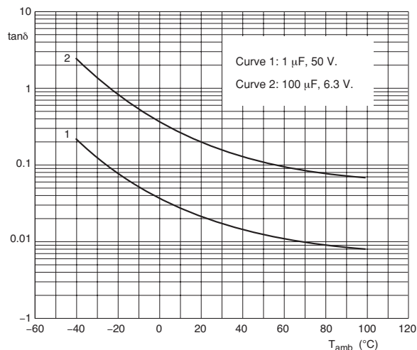
Fig.7 Typical dissipation factor ( \tan \delta ) at 100 or 120 Hz as a function of ambient temperature.
