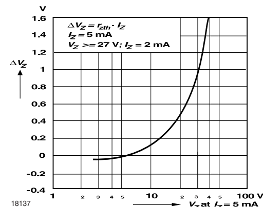
Fig. 14 Change of Zener voltage from turn-on up to the point of thermal equilibrium vs. Zener voltage
