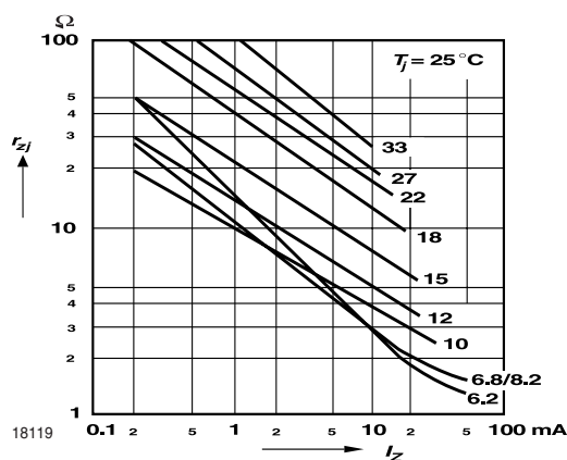
Fig. 6 Dynamic Resistance vs. Zener Current
