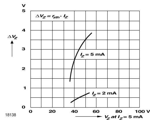
Fig. 15 Change of Zener voltage from turn-on up to the point of thermal equilibrium vs. Zener voltage
