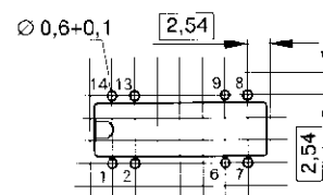
Mounting hole layout
