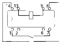
2 form a, standard
