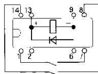
2 form a, with diode
