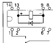
1 form c, with diode
