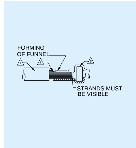
Figure 1 - Correct
