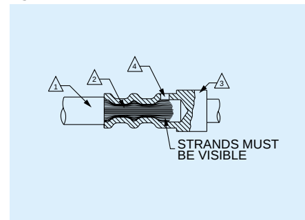
Figure 6 - Correct
