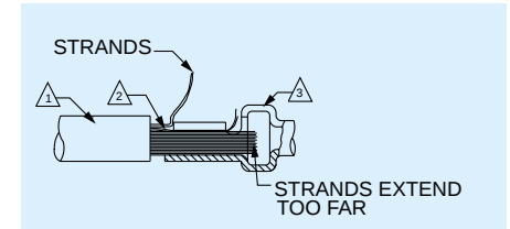
Figure 3 - Unacceptable
