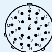
23 Way Shell Size 18
