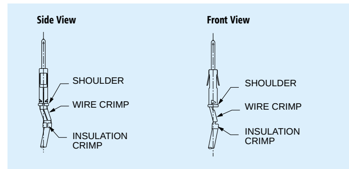
Figure 5 - Unacceptable
