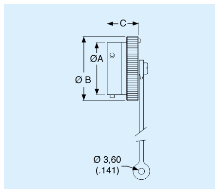
Plug Dust Cap
