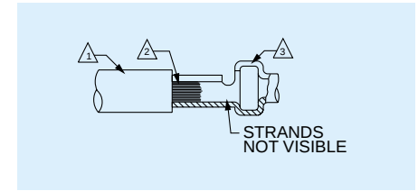
Figure 2 - Unacceptable
