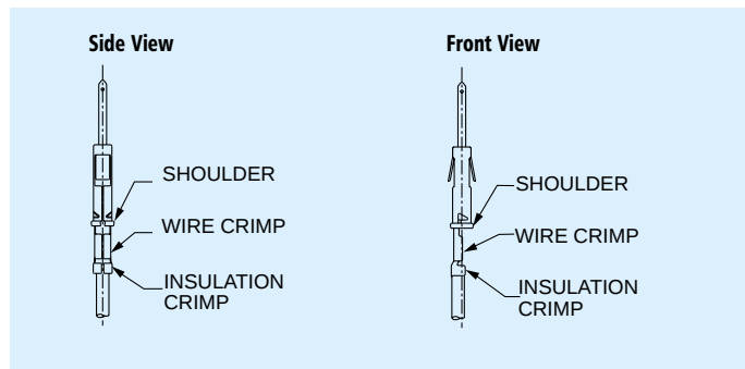
Figure 4 - Correct
