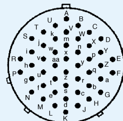
48 Way Shell Size 24
