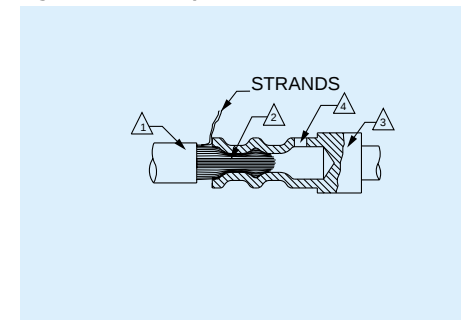
Figure 7 - Unacceptable
