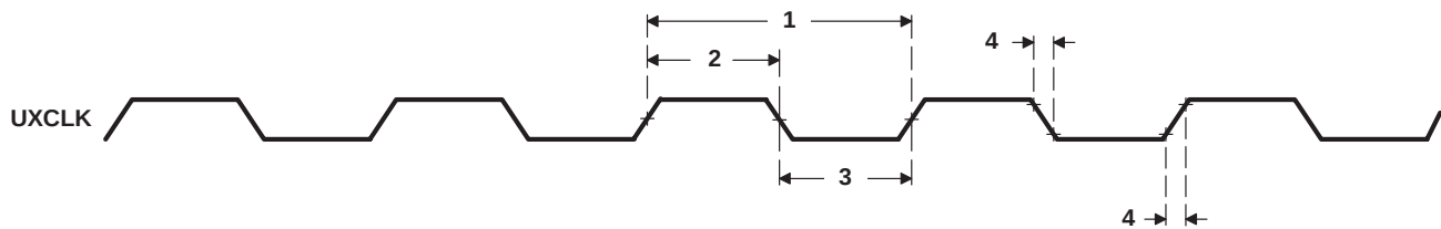
Figure 56. UXCLK Timing
