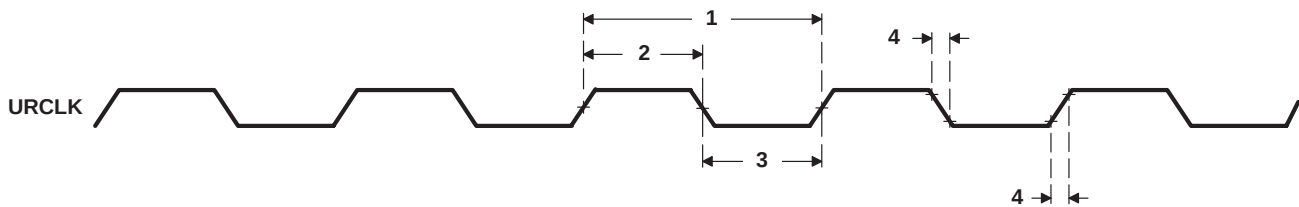
Figure 57. URCLK Timing
