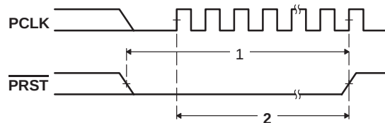
Figure 47. PCI Reset ( \overline{\text{PRST}} ) Timing
