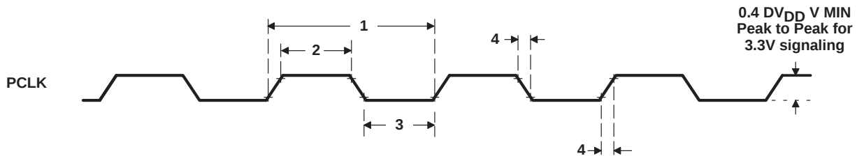
Figure 46. PCLK Timing
