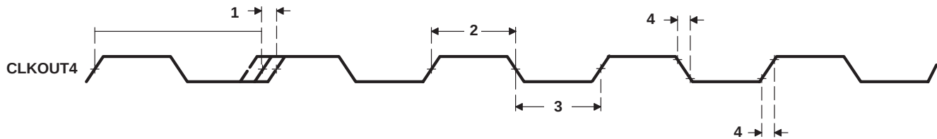
Figure 16. CLKOUT4 Timing
