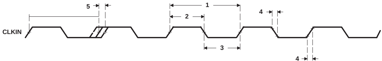
Figure 15. CLKIN Timing
