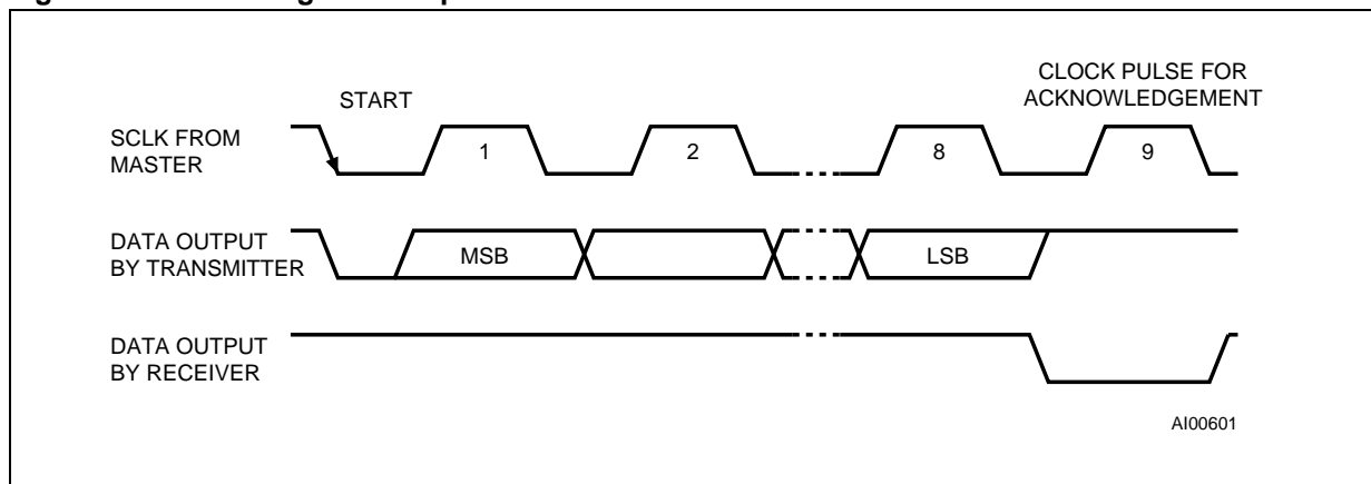
Figure 9. Acknowledgment Sequence
