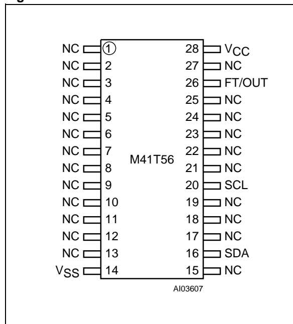
Figure 4. SOH28 Connections
