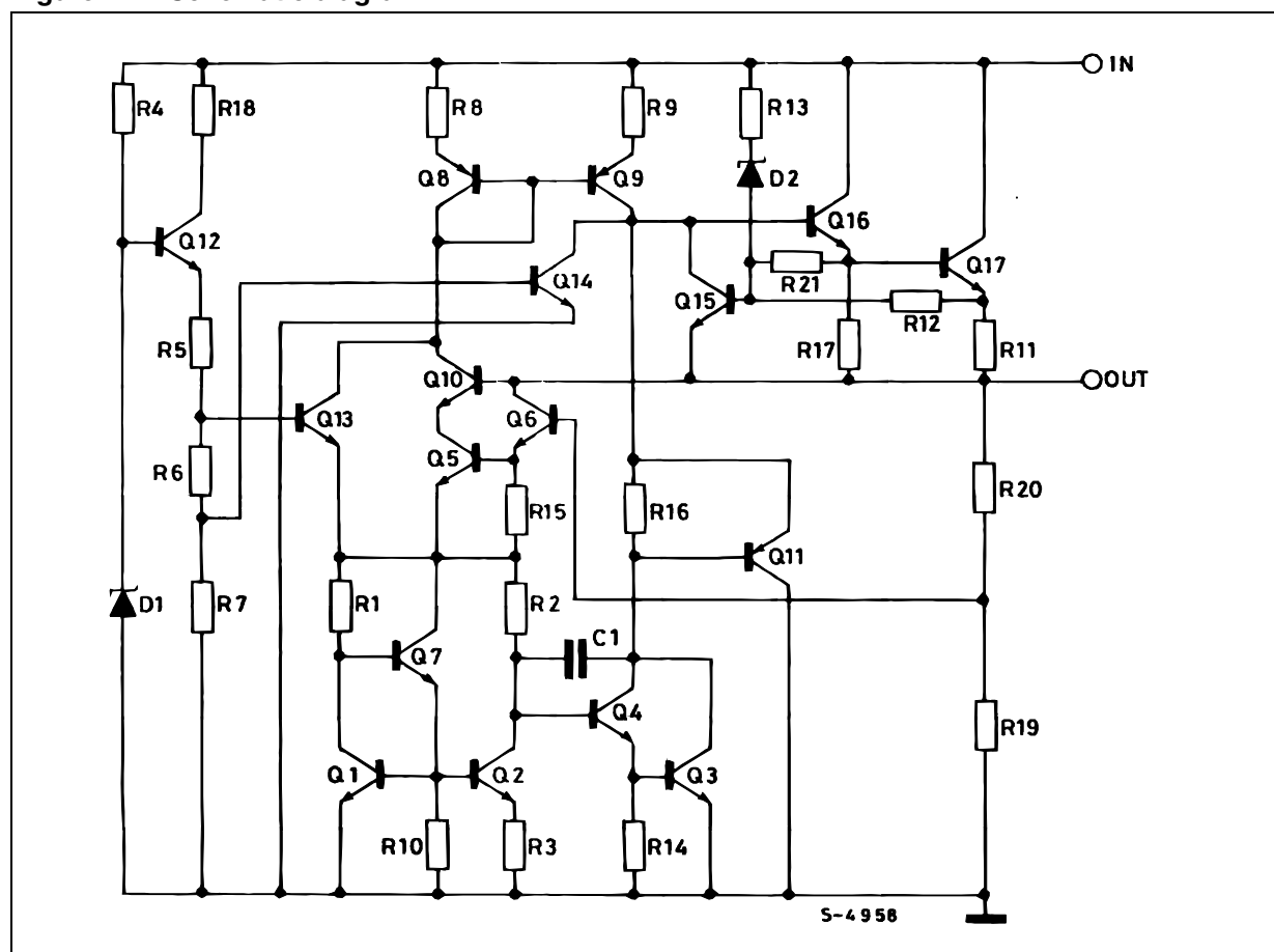
Figure 2. Schematic diagram
