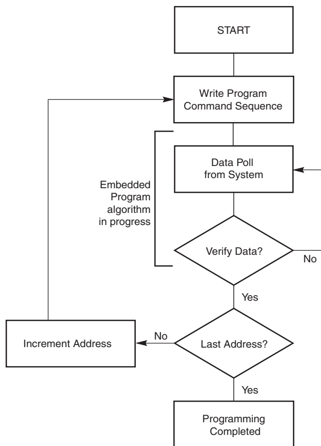
Figure 8.1 Program Operation
