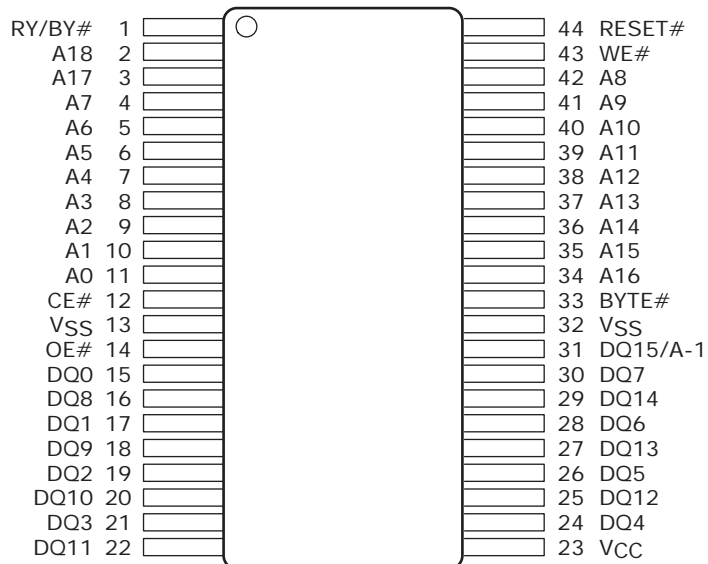
Figure 3.2 SO Pinout
