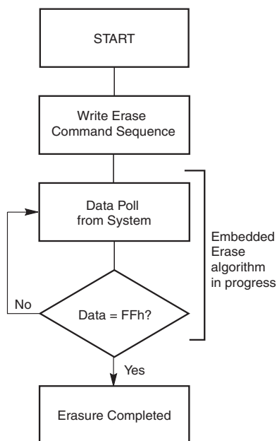
Figure 8.2 Erase Operation
