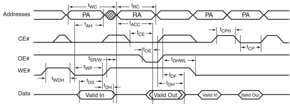
Figure 15.7 Back to Back Read/Write Cycle Timing
