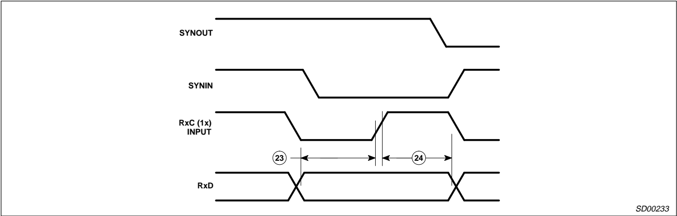
Figure 10. Receive Timing
