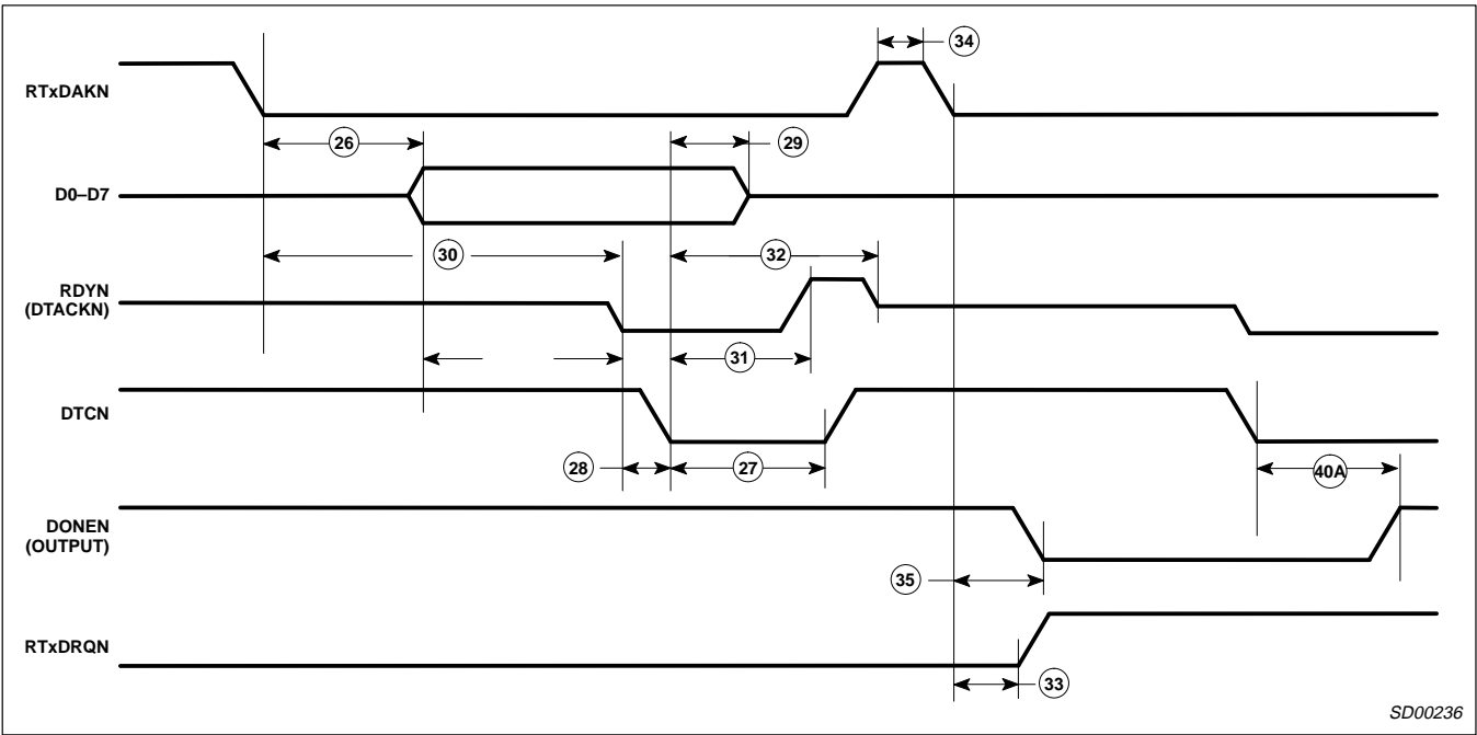
Figure 13. DMA Receive Read Timing—Single Address DMA Mode
