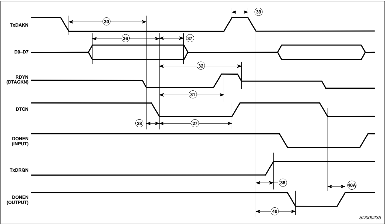
Figure 12. DMA Transmit Write Timing—Single Address DMA Mode
