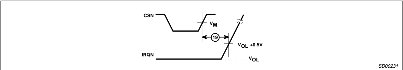
Figure 7. Interrupt Timing
