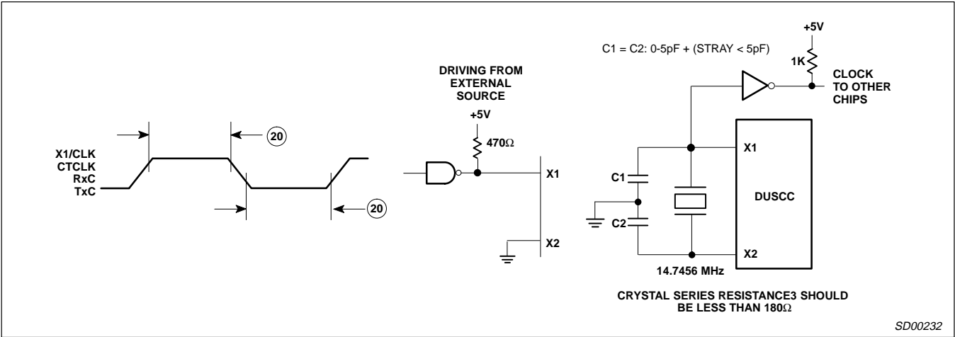
Figure 8. Clock Timing
