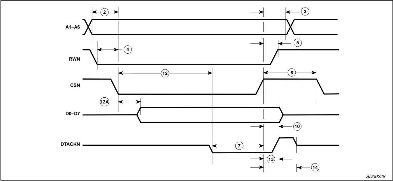
Figure 4. Bus Timing (Write Cycle)
