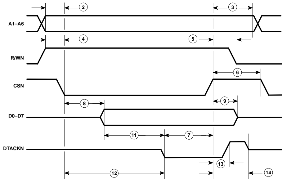
Figure 2. Bus Timing (Read Cycle)
