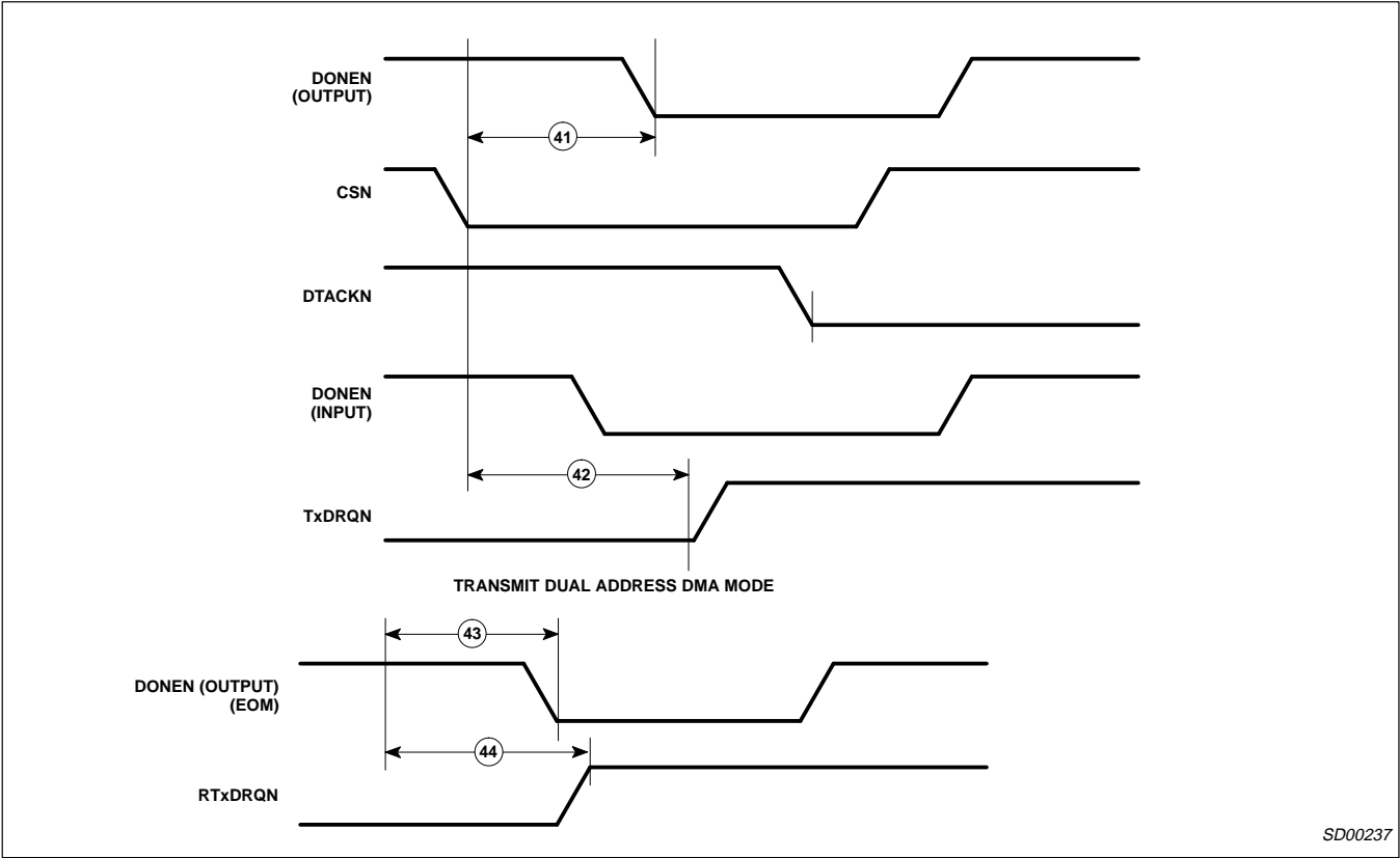
Figure 14. Dual Address DMA Mode Timing
