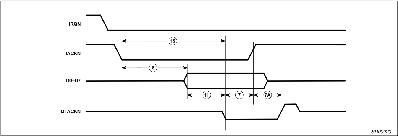
Figure 5. Interrupt Cycle Timing
