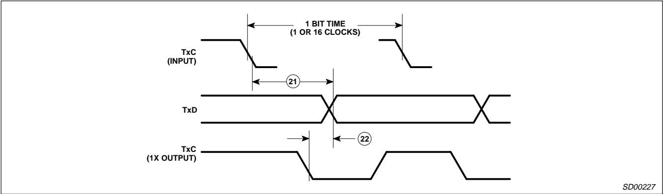
Figure 9. Transmit Timing
