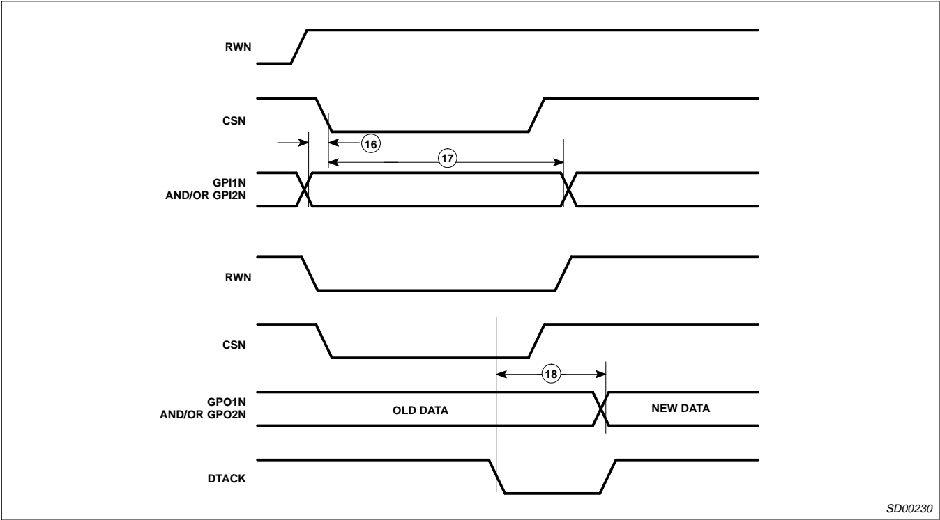
Figure 6. Port Timing
