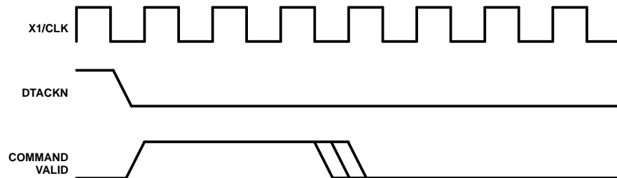
Figure 3. Command Timing
