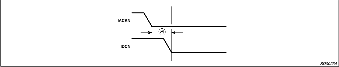
Figure 11. Interrupt Daisy Chain Timing
