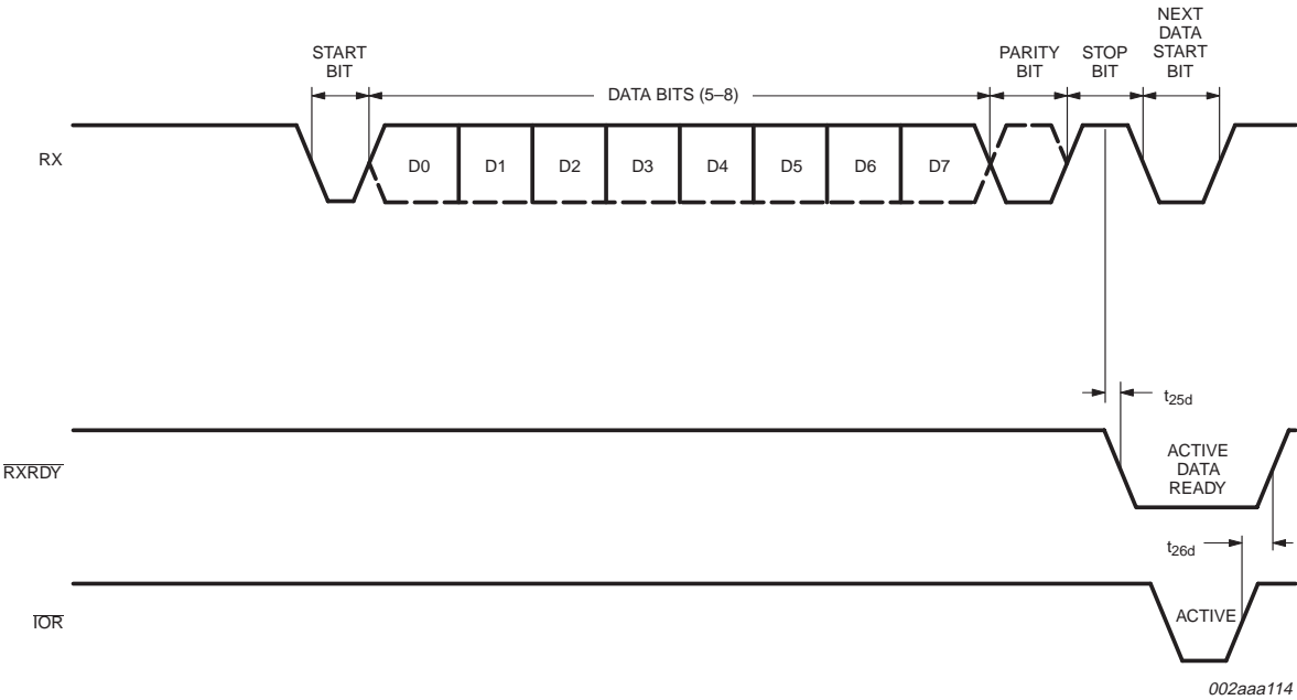
Fig 16. Receive ready timing in non-FIFO mode.
