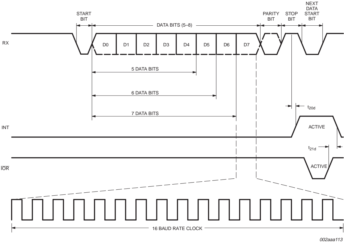
Fig 15. Receive timing.
