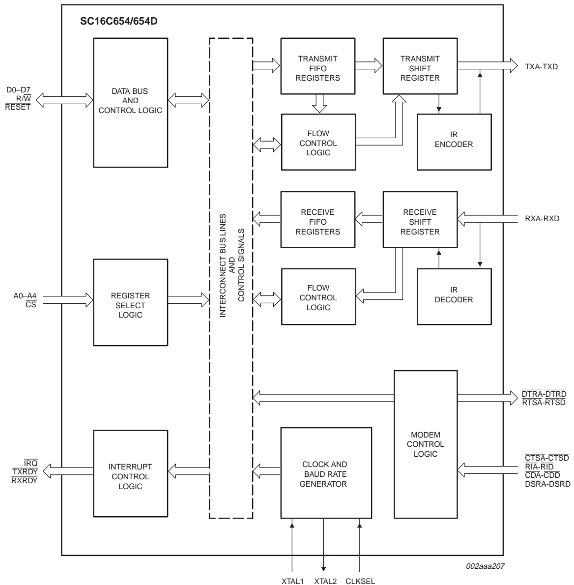
Fig 2. SC16C654/654D block diagram (68 mode).
