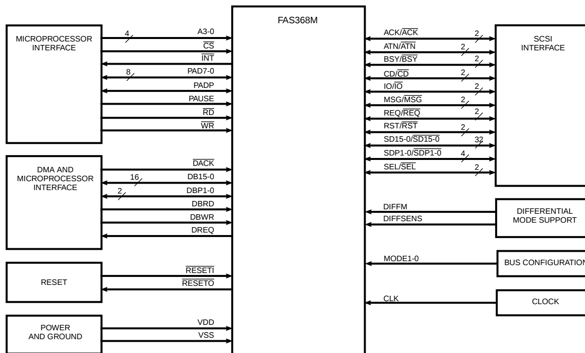
Figure 4. FAS368M Functional Signal Grouping
