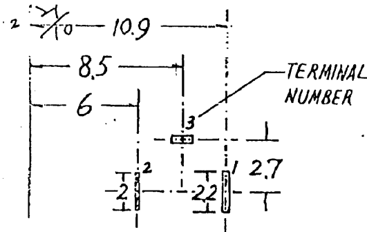
SETTING OUT OF P.C. BOARD
