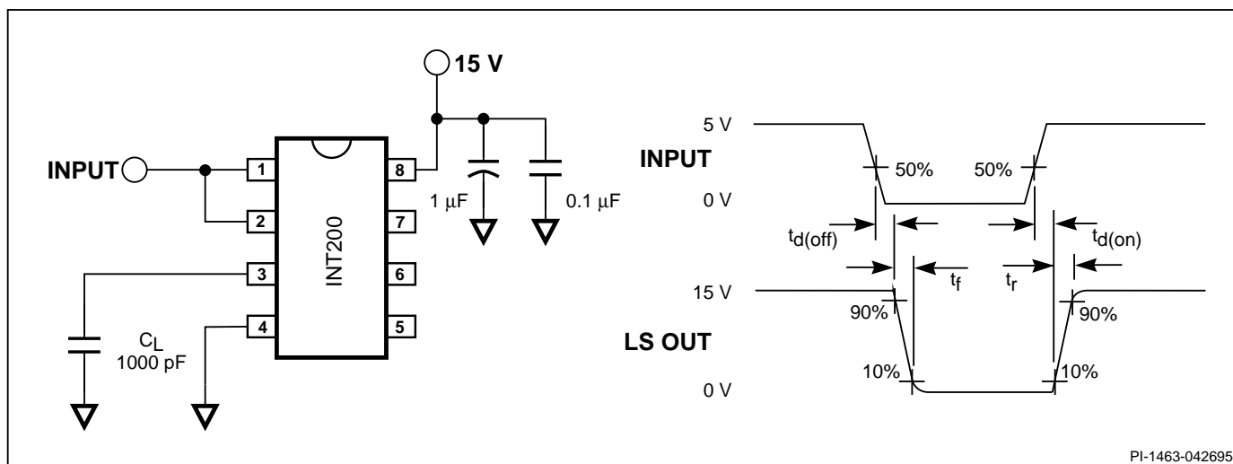
Figure 7. Switching Time Test Circuit.
