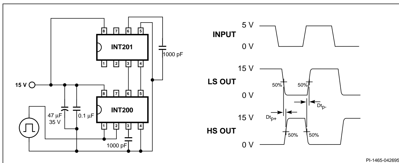
Figure 8. Dead Time Test Circuit.
