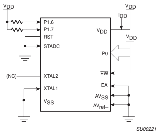
Figure 61. I DD Test Condition, Power Down Mode All other pins are disconnected. V_{DD} = 2 \text{ V to } 5.5 \text{ V}^3
