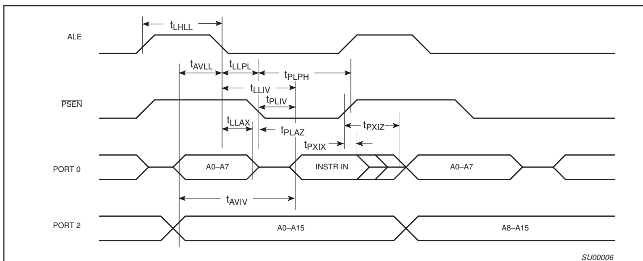
Figure 49. External Program Memory Read Cycle
