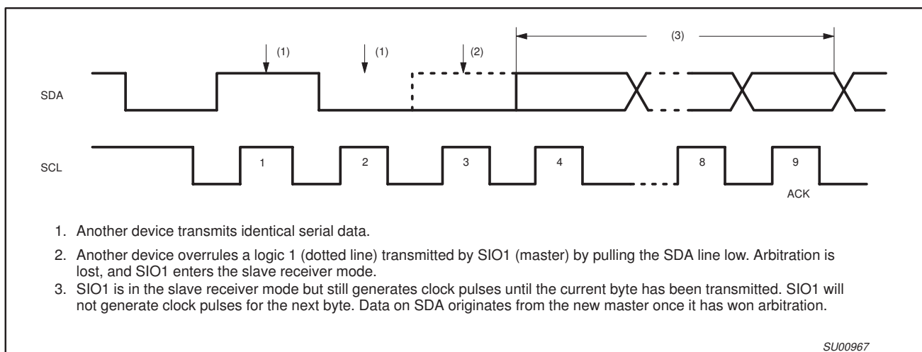
Figure 36. Arbitration Procedure
