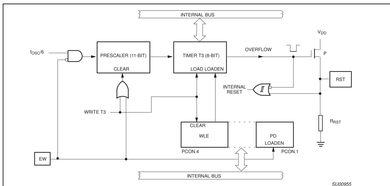
Figure 18. Watchdog Timer
