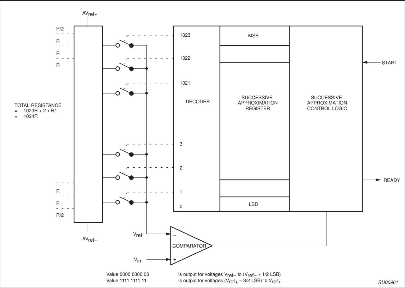
Figure 24. ADC Realization
