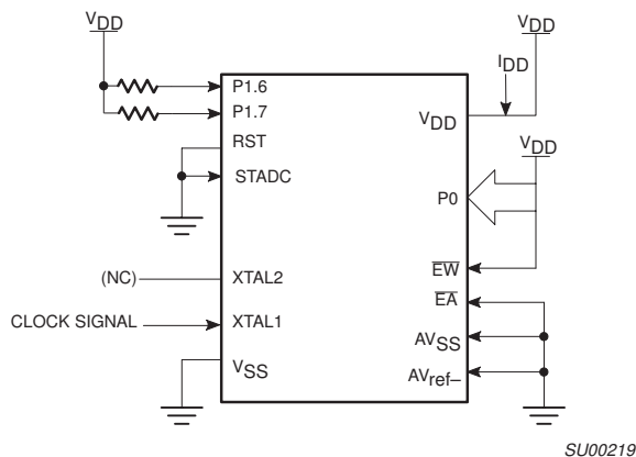
Figure 59. I DD Test Condition, Idle Mode All other pins are disconnected 2
