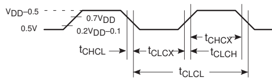
Figure 60. Clock Signal Waveform for I DD Tests in Active and Idle Modes t_{CLCH} = t_{CHCL} = 5 \text{ ns}
