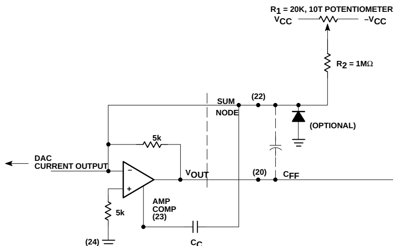
Figure 14. Zero-Scale Adjustment
