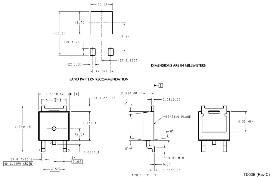
TO-252 Package (DT) NS Package Number TD03B
