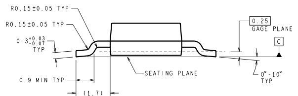
SOT-223 Package (MP) NS Package Number MP04A
