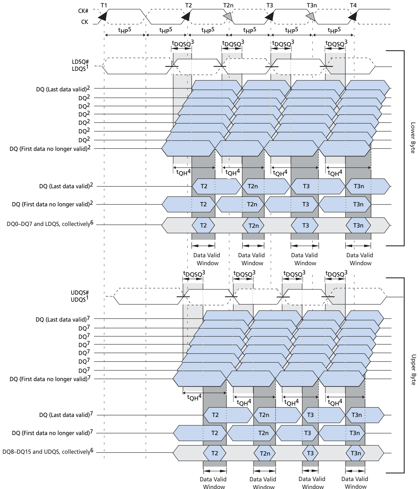
Figure 30: x16 Data Output Timing – t_{DQSQ} , t_{QH} , and Data Valid Window Figure notes appear on page 52
