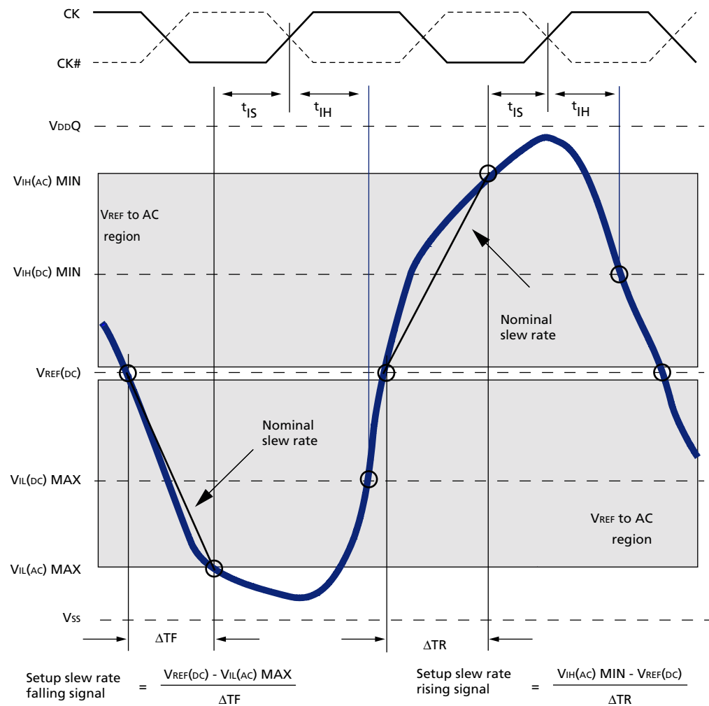
Figure 69: Nominal Slew Rate for t_{IS}
