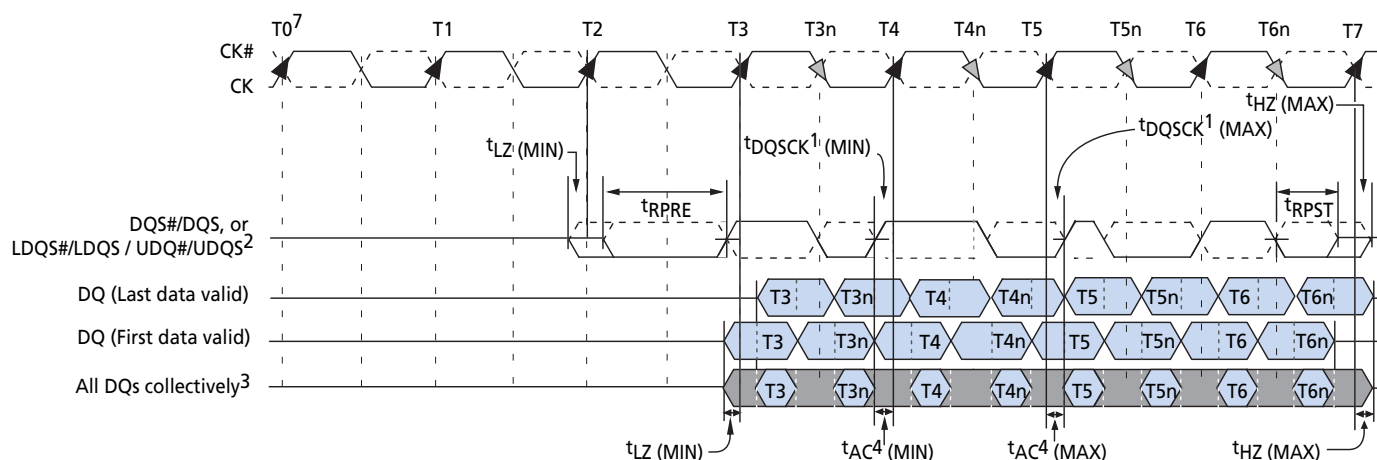
Figure 31: Data Output Timing – t_{AC} and t_{DQSCK}
