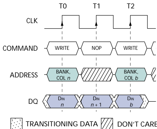
Figure 15 WRITE to WRITE
