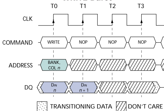
Figure 14 WRITE Burst
