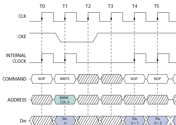
Figure 22 Clock Suspend During WRITE Burst
