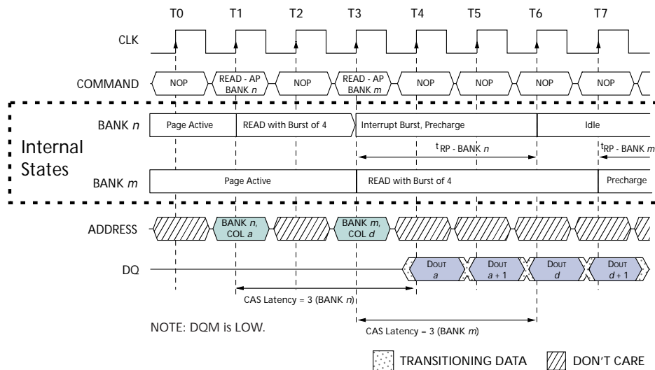
Figure 24 READ With Auto Precharge Interrupted by a READ
