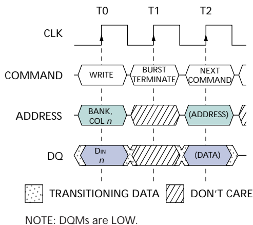
Figure 19 Terminating a WRITE Burst
