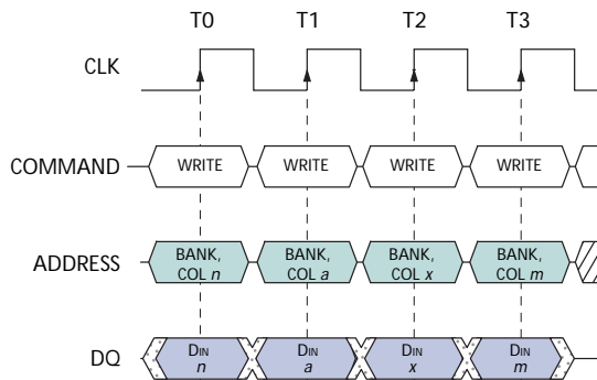
Figure 16 Random WRITE Cycles
