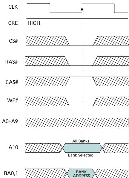
Figure 20 PRECHARGE Command
