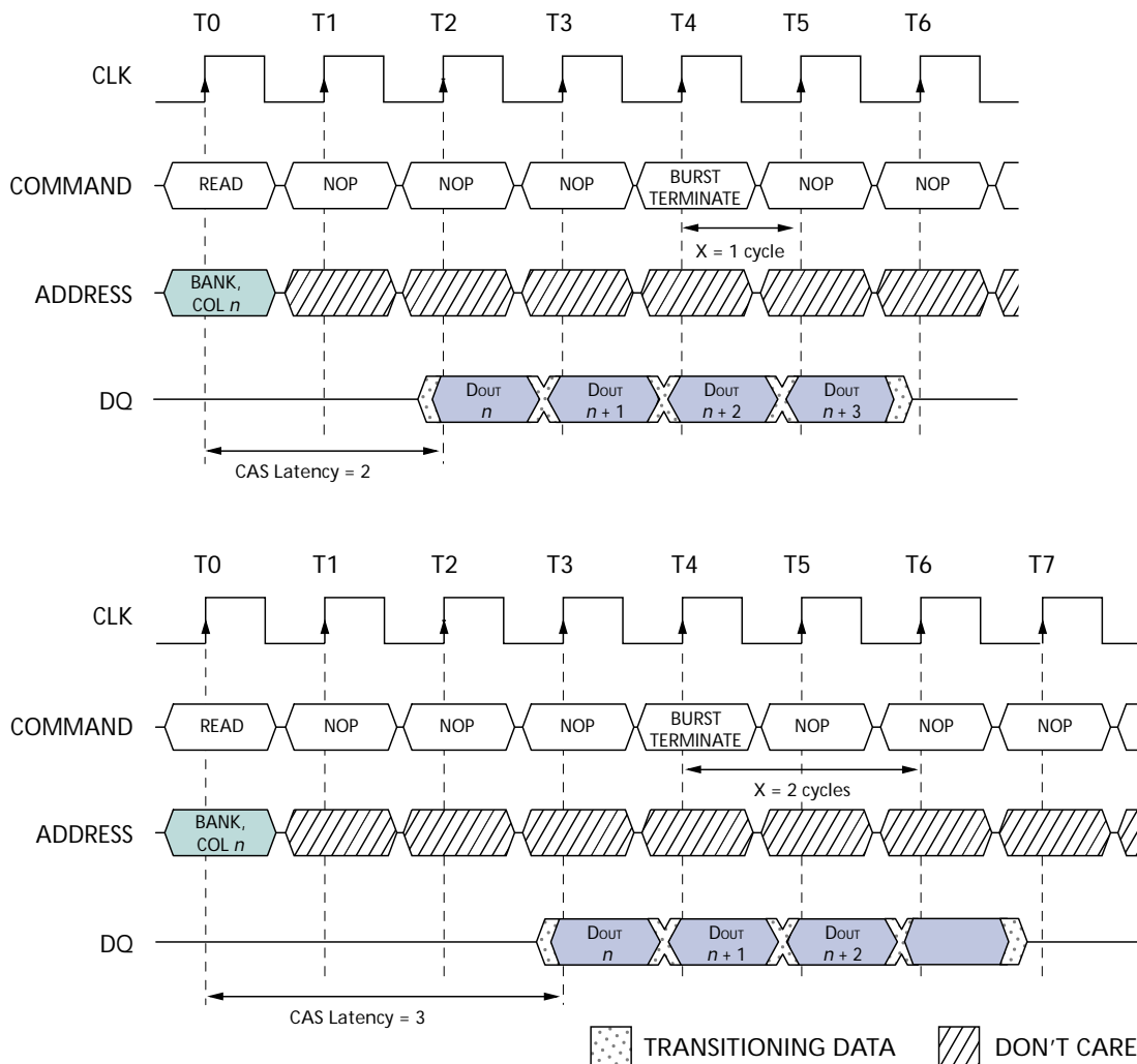
Figure 12 Terminating a READ Burst
