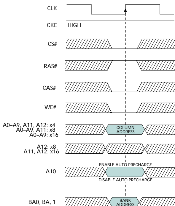
Figure 13 WRITE Command
