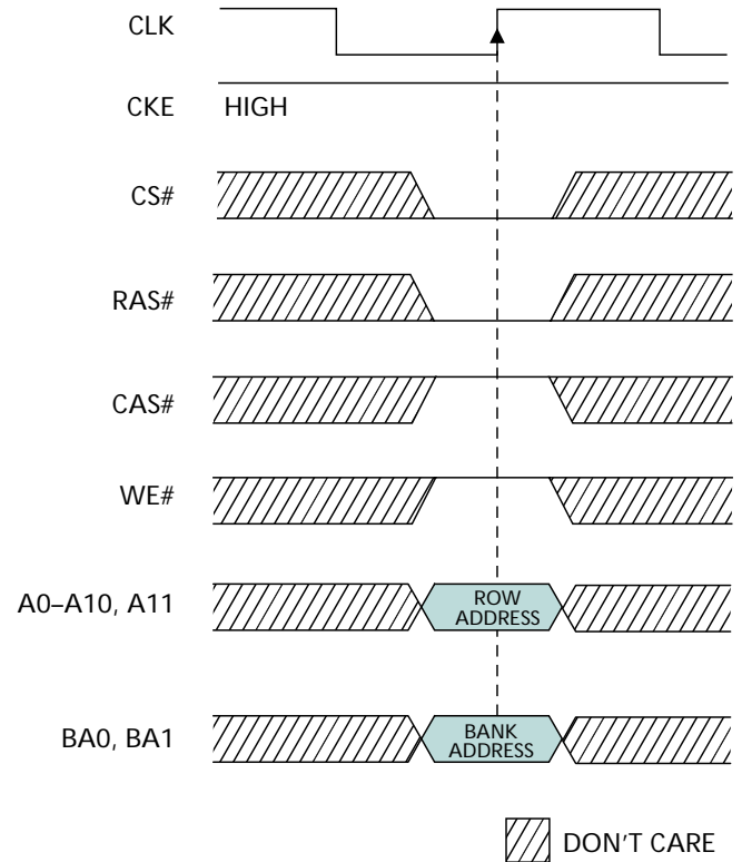
Figure 4 Example: Meeting t_{RCD} (MIN) When 2 < t_{RCD} \text{ (MIN)} / t_{CK} \leq 3
