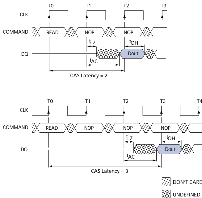
Figure 2 CAS Latency
