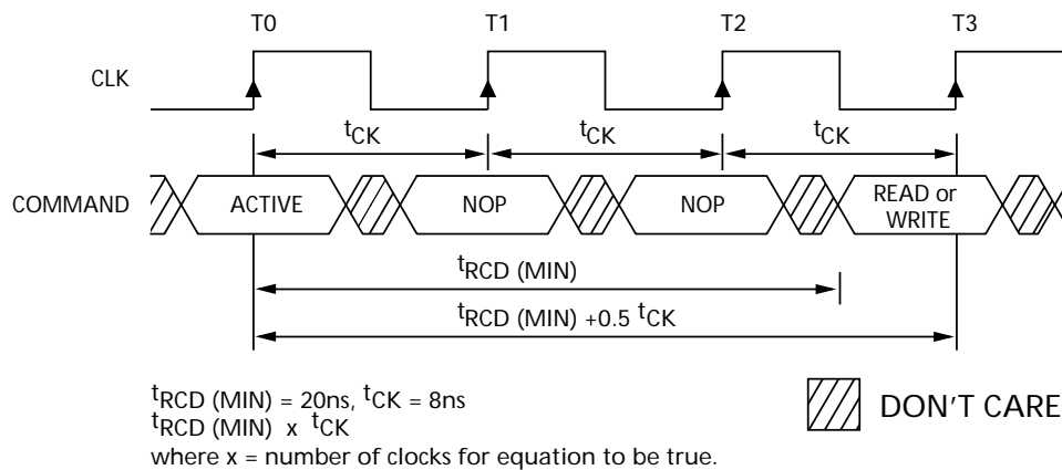
Figure 4 Example: Meeting t_{\text{RCD}} \text{ (MIN)} When 2 < t_{\text{RCD}} \text{ (MIN)} / t_{\text{CK}} - 3
