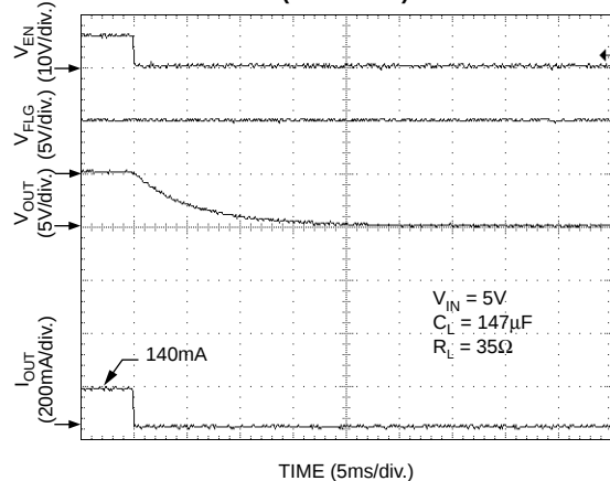
Turnoff (MIC2027-1)
