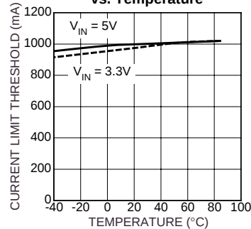
Current-Limit Threshold vs. Temperature
