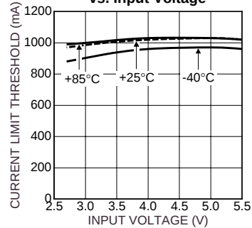
Current-Limit Threshold vs. Input Voltage
