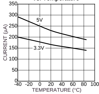
Supply On-Current vs. Temperature
