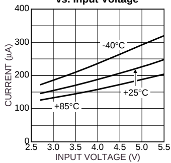
Supply On-Current vs. Input Voltage
