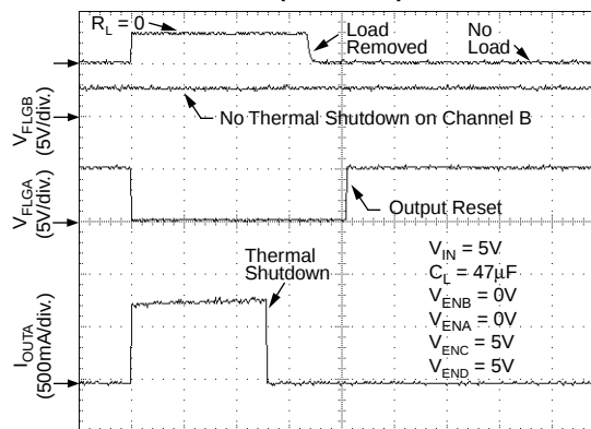
Independent Thermal Shutdown (MIC2077-2)
