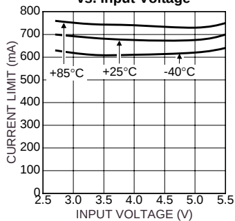
Short-Circuit Current-Limit vs. Input Voltage
