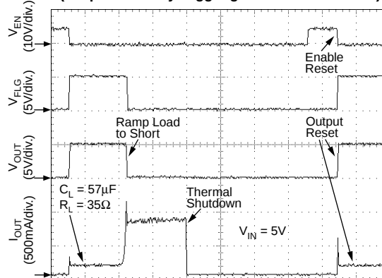
Thermal Shutdown (Output Reset by Toggling Enable—MIC2077-2)
