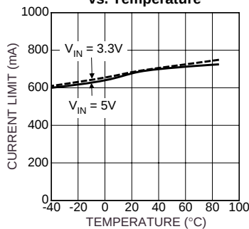
Short-Circuit Current-Limit vs. Temperature
