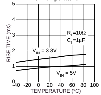
Turn-On Rise Time vs. Temperature
