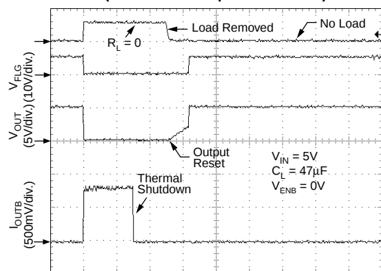
Thermal Shutdown (MIC2077-2—Output Latched Off)
