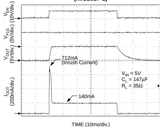
Turn-On/Turnoff (MIC2027-1)
