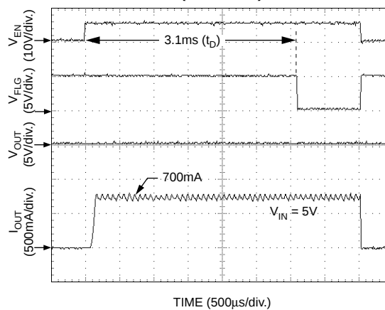
Enabled Into Short (MIC2027-1)
