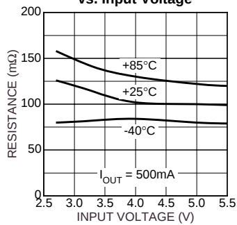
On-Resistance vs. Input Voltage
