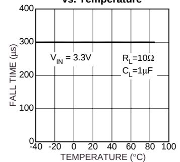
Fall Time vs. Temperature
