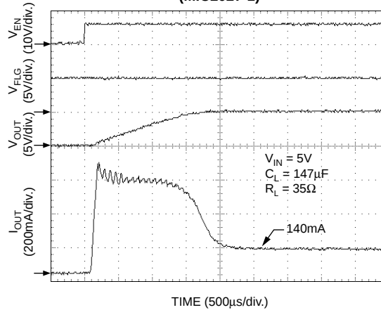
Turn-On (MIC2027-1)
