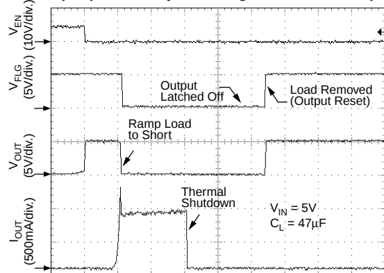
Thermal Shutdown (Output Reset by Removing Load—MIC2077-2)
