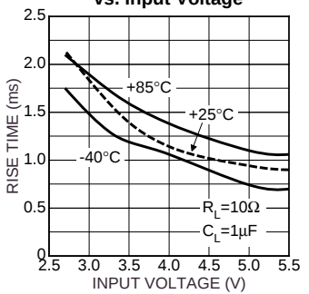
Turn-Off Rise Time vs. Input Voltage
