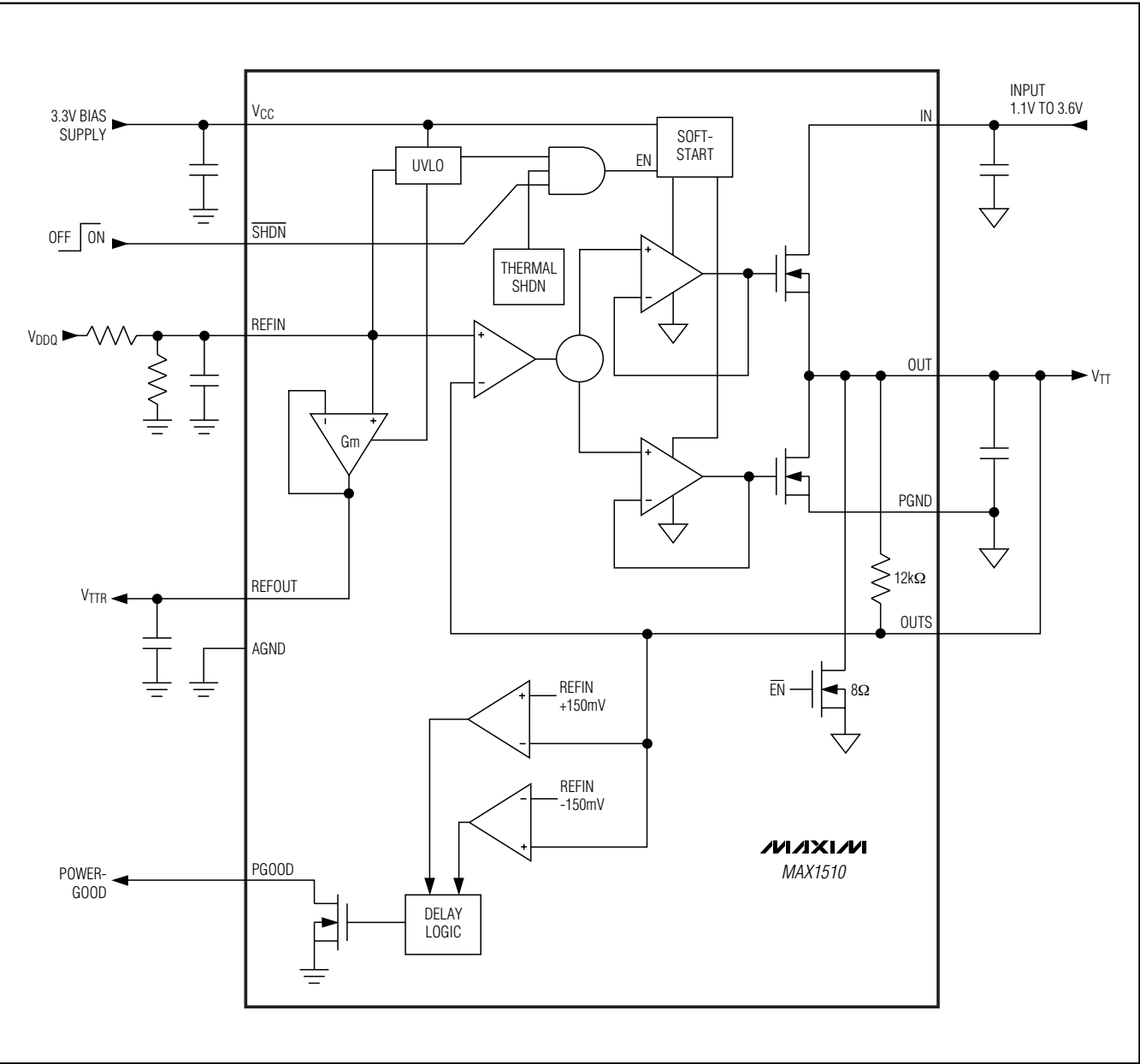
Figure 2. Functional Diagram
