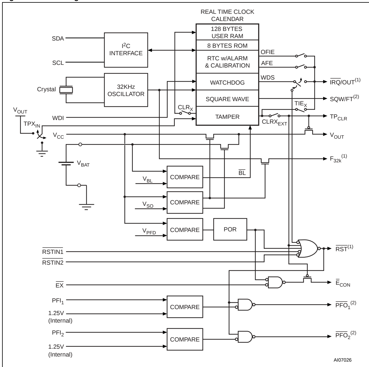
Figure 4. Block Diagram
