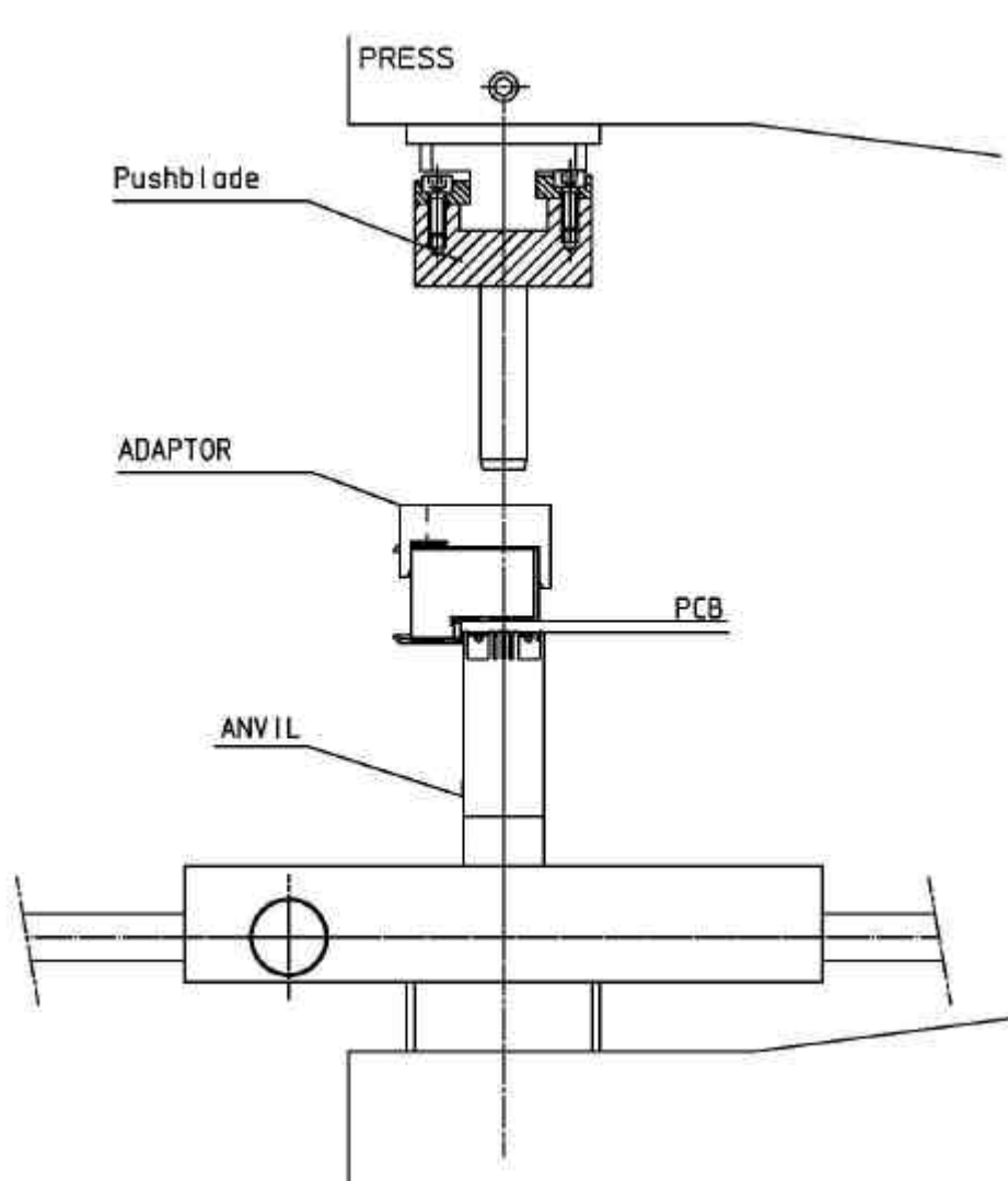
Figure 10 – Application Tooling Overview
