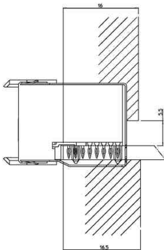
Figure 6 -- Keep-out Zones
