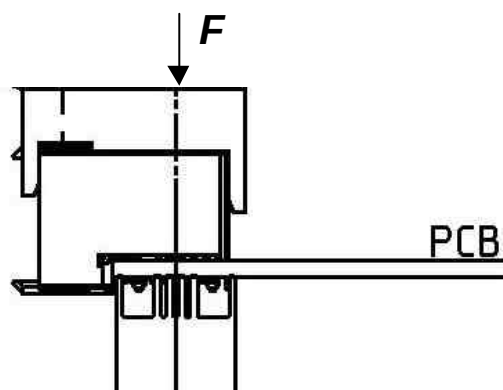
Figure 12 – Applying Force
