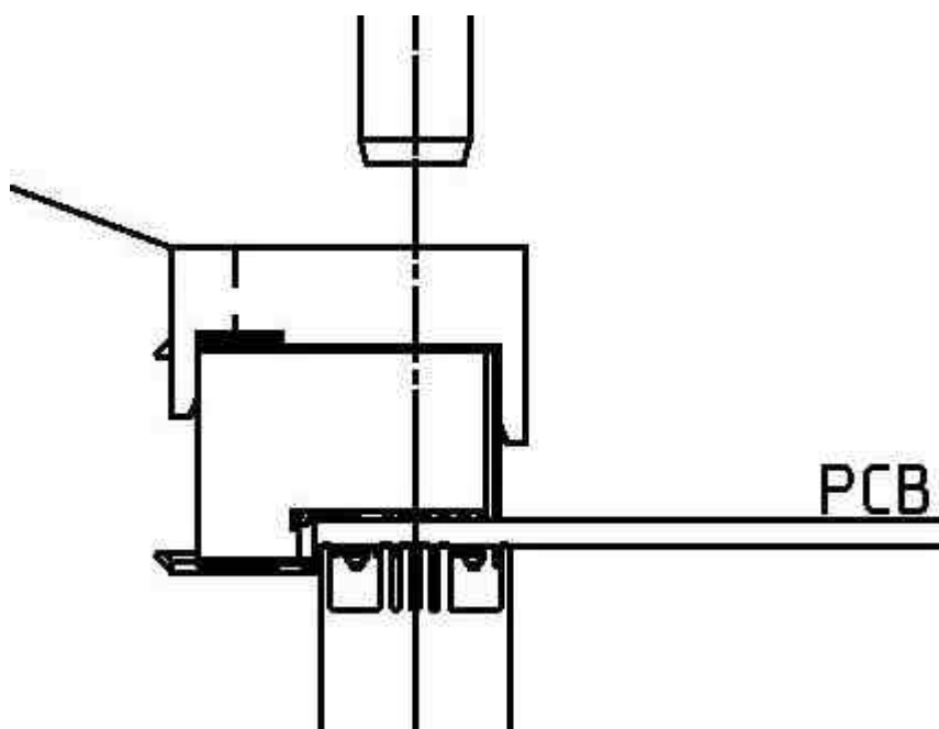
Figure 11 – Insertion Procedure
