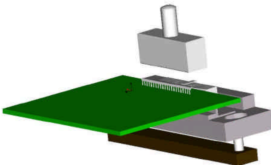
Figure 15 - One Piece Cover Shield Tool HM2Y509
