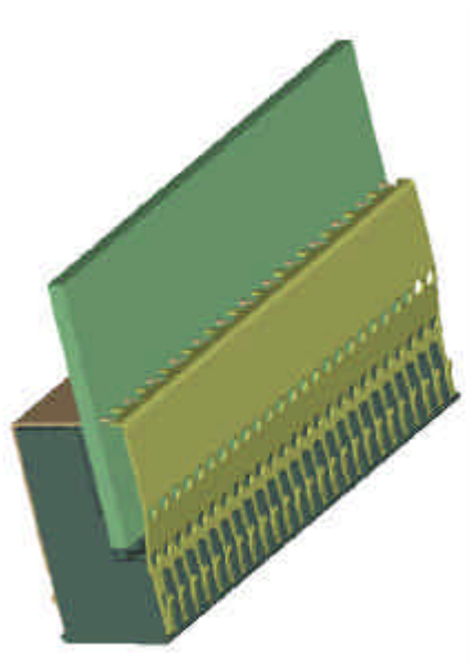
Figure 14 – One piece cover shield
