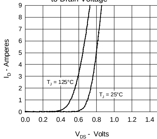
Fig.10 Source Current vs. Source to Drain Voltage
