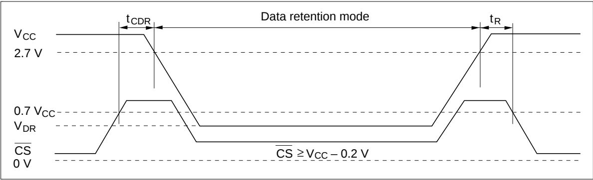
Low V_{CC} Data Retention Timing Waveform ( \overline{CS} Controlled)
