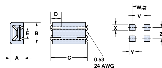
Figure 4 Common-Mode Bead
