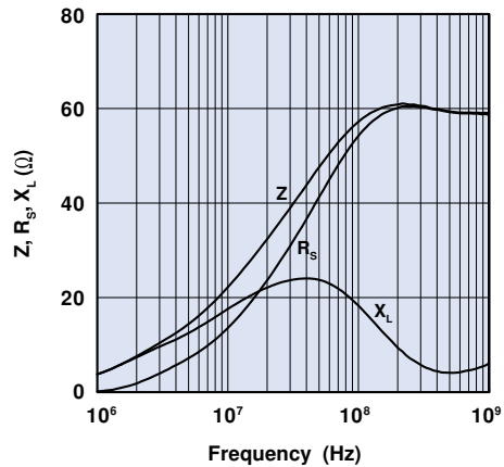
Figure 19A Impedance, reactance, and resistance vs. frequency for SM bead 2744040447.
