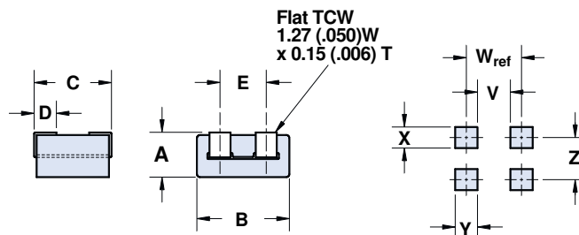
Figure 2 Common-Mode Bead
