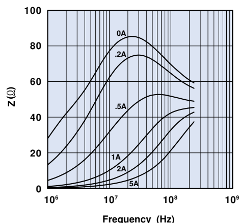
Figure 10B Impedance vs. frequency with dc bias as parameter for SM bead 2773021447.
