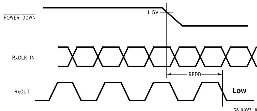
FIGURE 13. Receiver Powerdown Delay
