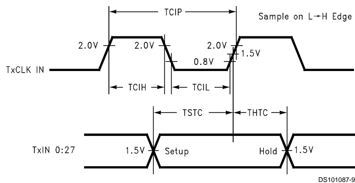
FIGURE 5. DS90CR287 (Transmitter) Setup/Hold and High/Low Times
