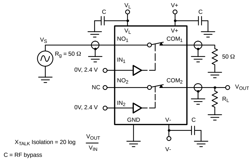
FIGURE 5. Crosstalk
