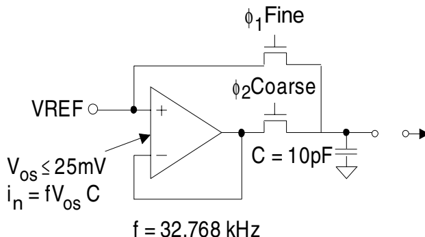
Figure 2. Input model for VREF+ and VREF- pins.
