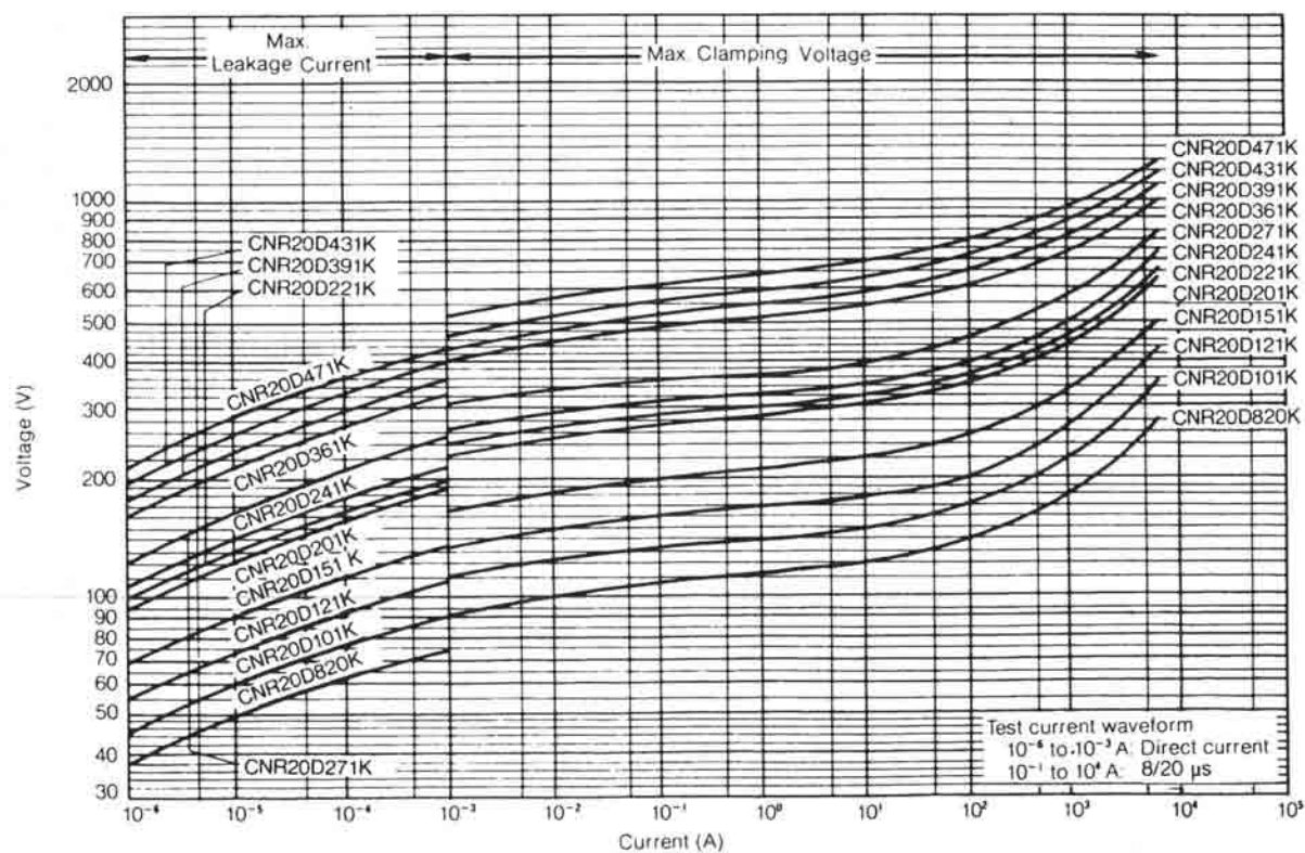
V-I Curve (CNR20D820K to CNR20D471K)
