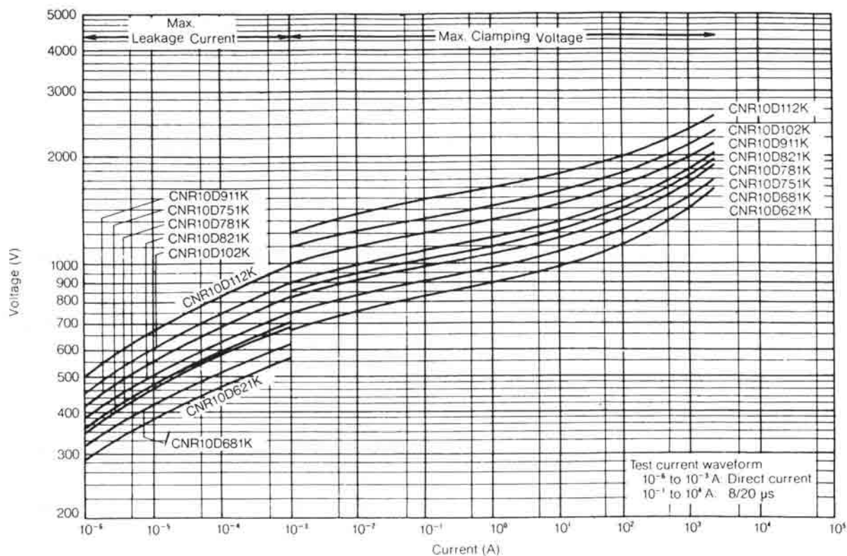
V-I Curve (CNR10D621K to CNR10D112K)
