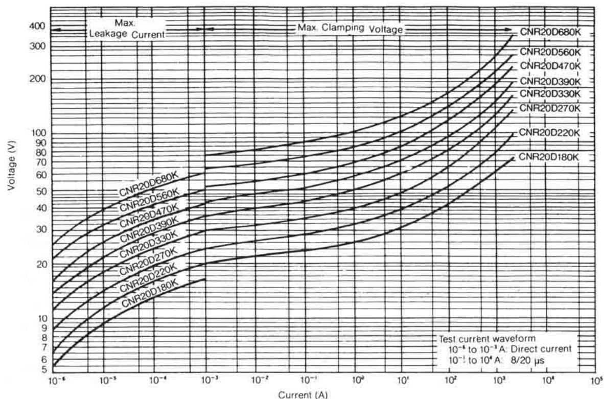
V-I Curve (CNR20D180K to CNR20D680K)
