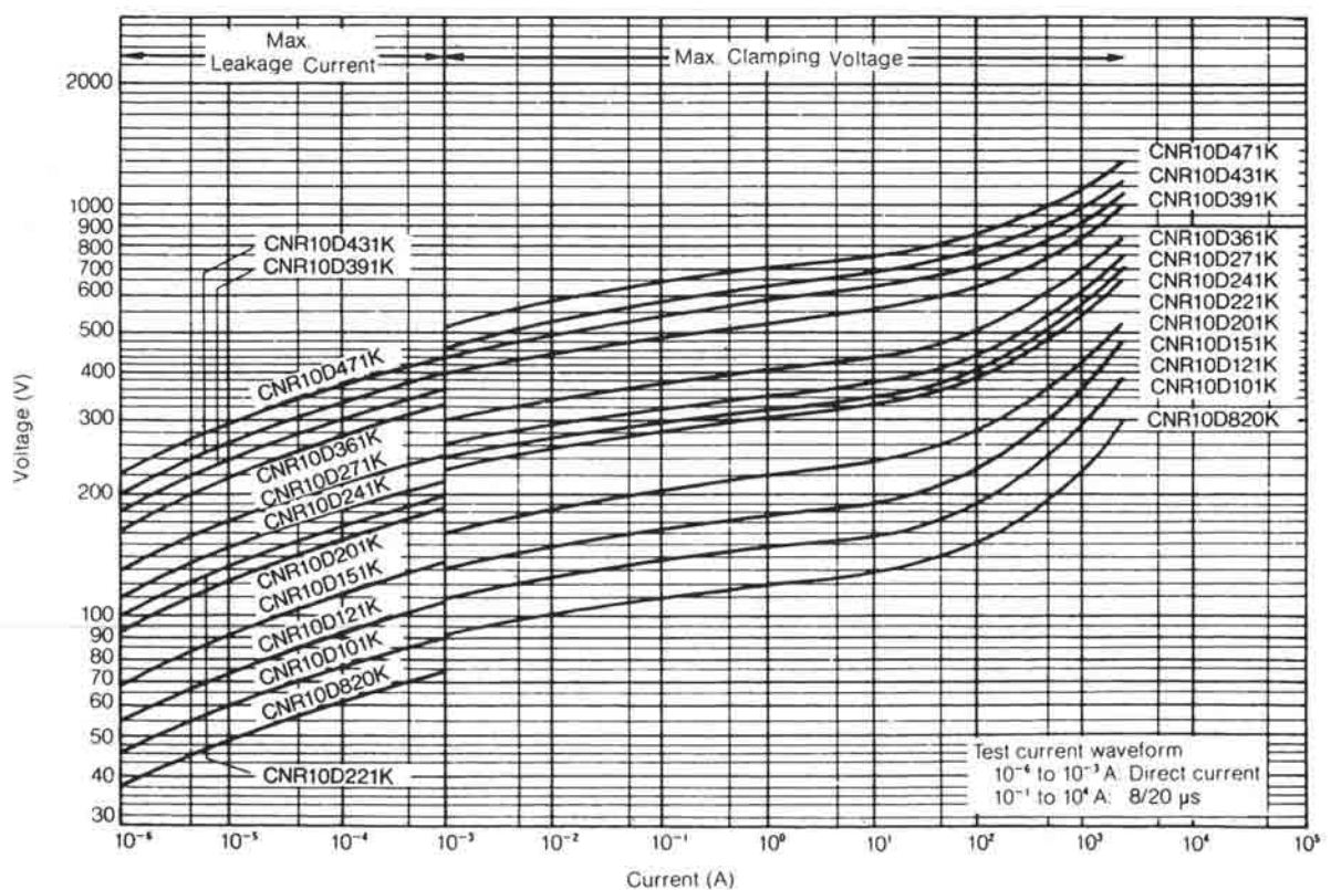
V-I Curve (CNR10D820K to CNR10D471K)
