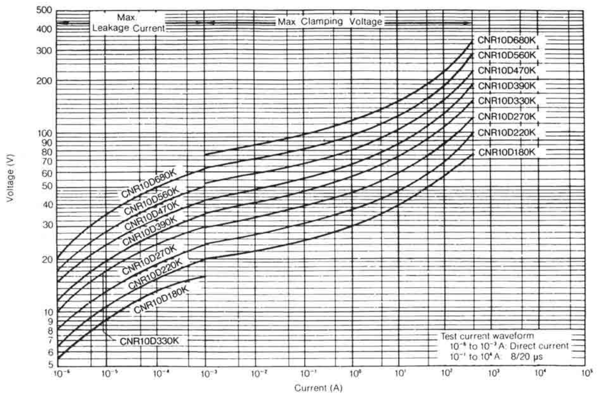
V-I Curve (CNR10D180K to CNR10D680K)
