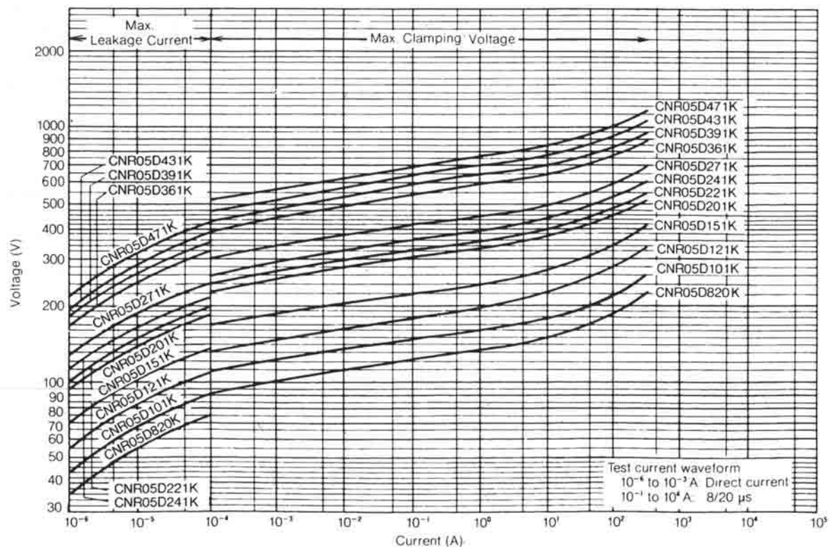
V-I Curve (CNR05D820K to CNR05D471K)
