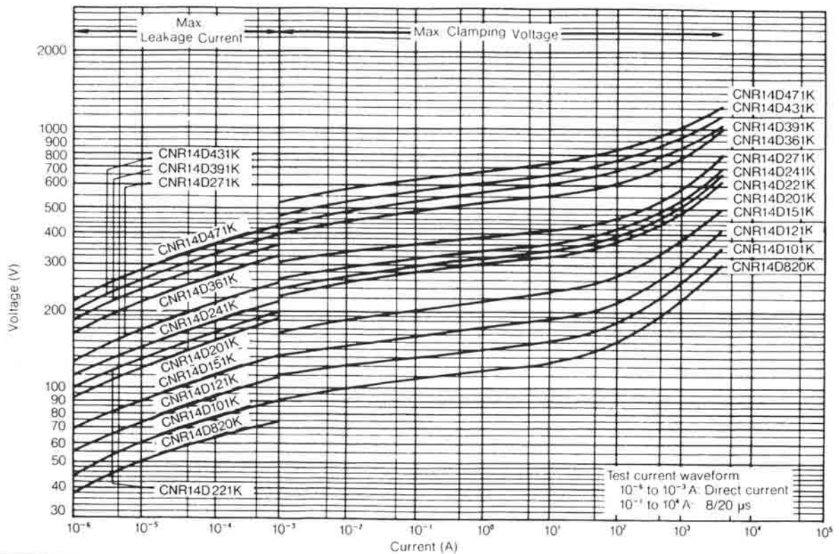
V-I Curve (CNR14D820K to CNR14D471K)
