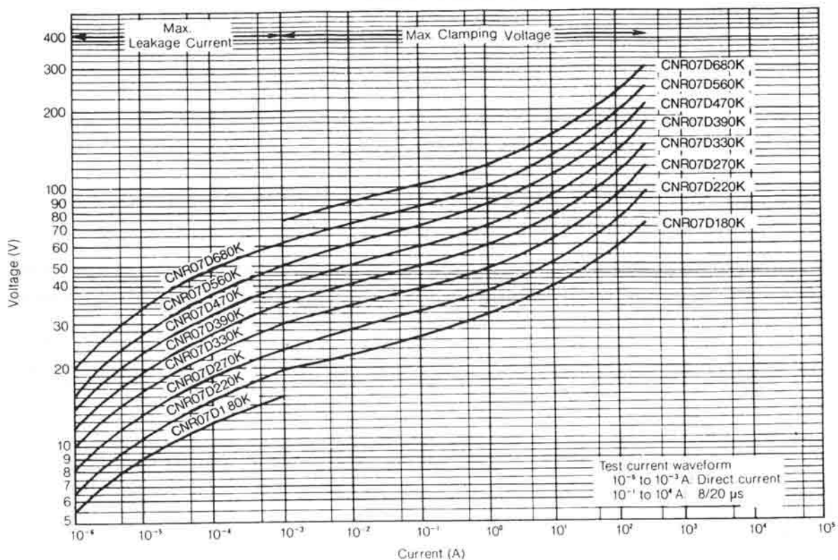
V-I Curve (CNR07D180K to CNR07D680K)
