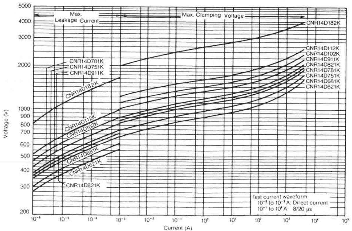
V-I Curve (CNR14D621K to CNR14D182K)
