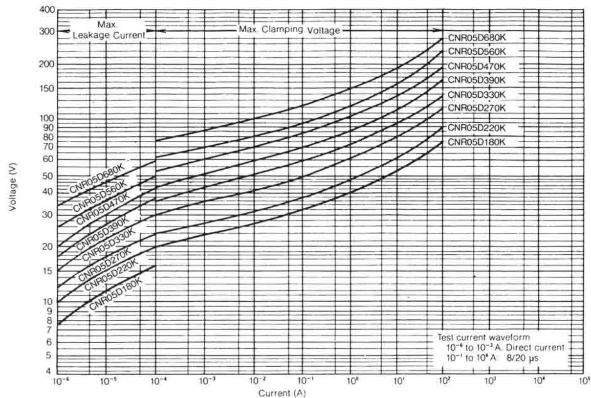
V-I Curve (CNR05D180K to CNR05D680K)
