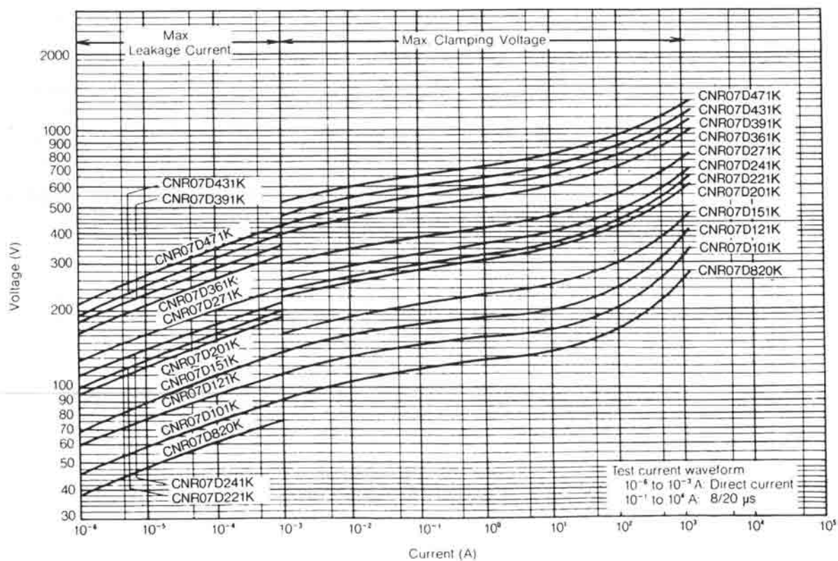
V-I Curve (CNR07D820K to CNR07D471K)
