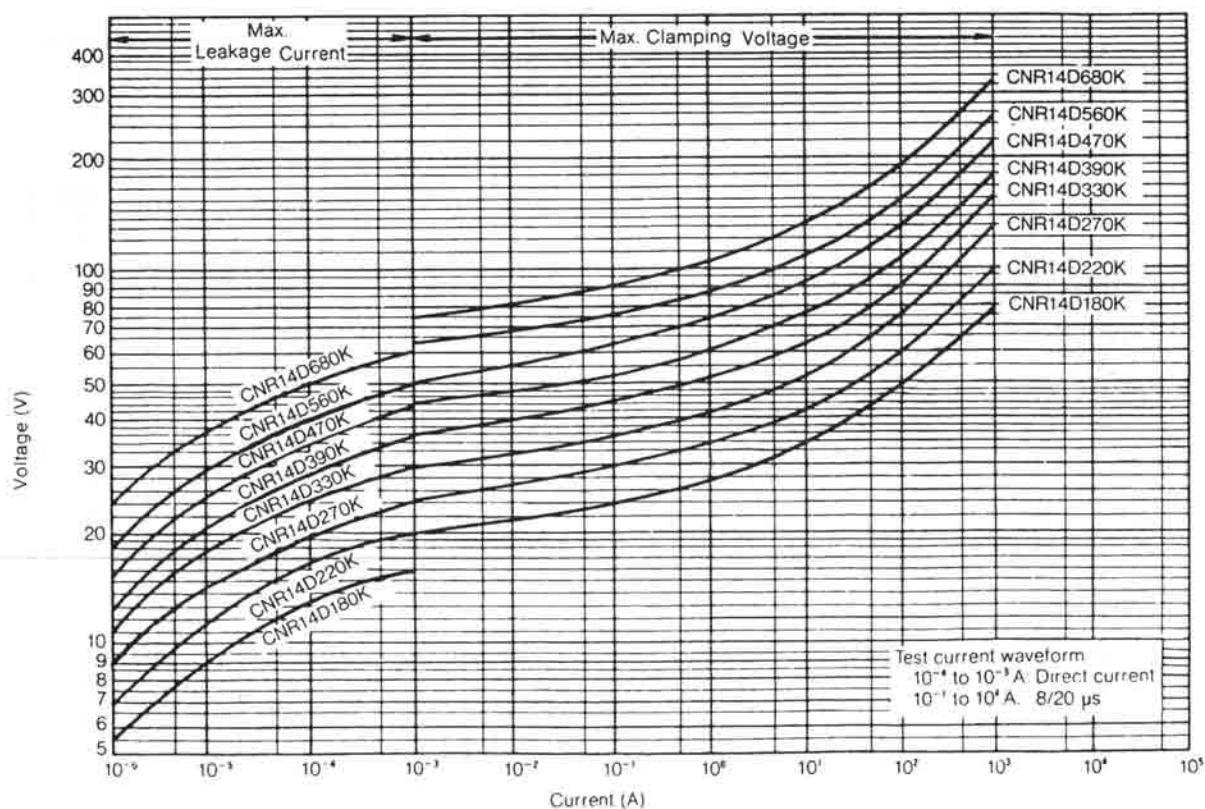
V-I Curve (CNR14D180K to CNR14D680K)
