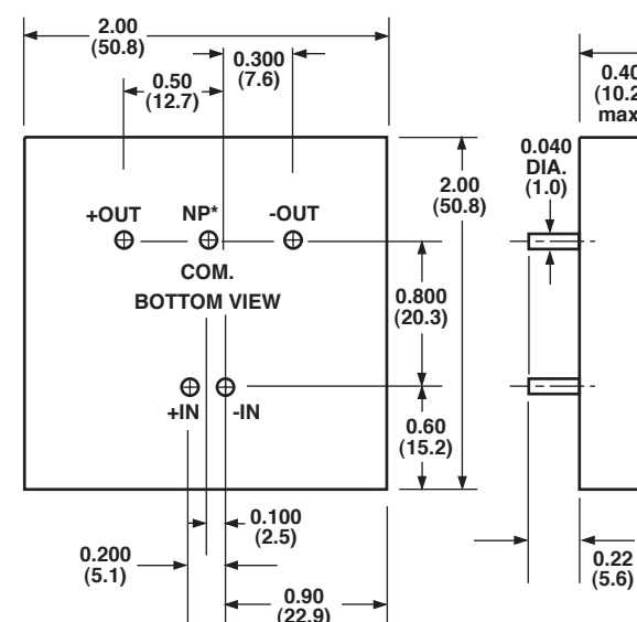
STANDARD PIN CONFIGURATION
