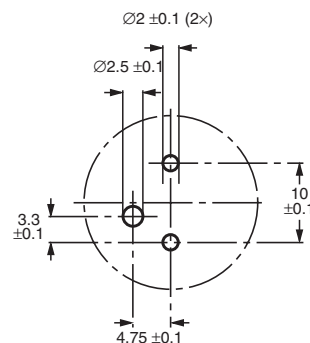
Fig.3 Mounting hole diagram.
