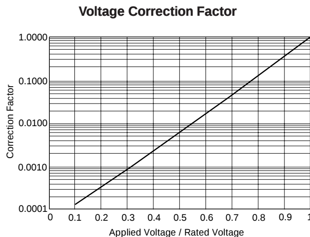
Figure 2. Correction factor to failure rate F for voltage derating of a typical component (60% con. level).
