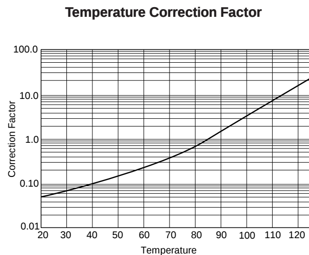
Figure 3. Correction factor to failure rate F for ambient temperature T for typical component (60% con. level).
