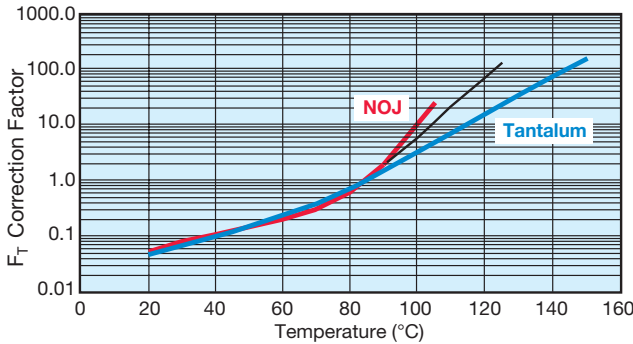
Figure 3: Correction factor to failure rate F for ambient temperature T for typical component (60% con. level).
