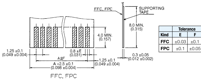
MOUNTING LAYOUT
