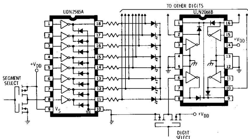
COMMON-CATHODE LED DRIVER
