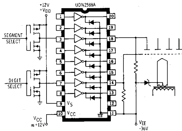
VACUUM-FLUORESCENT DISPLAY DRIVER (Split Supply)
