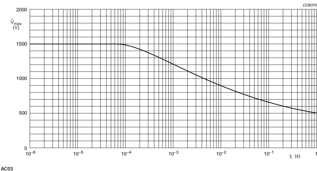
Fig.7 Pulse on a regular basis; maximum permissible peak pulse voltage ( \hat{V}_{\max} ) as a function of pulse duration ( t_i ).
