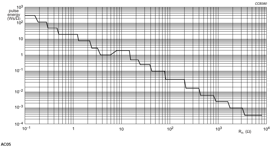
Fig.12 Pulse capability; W_s as a function of R_n .
