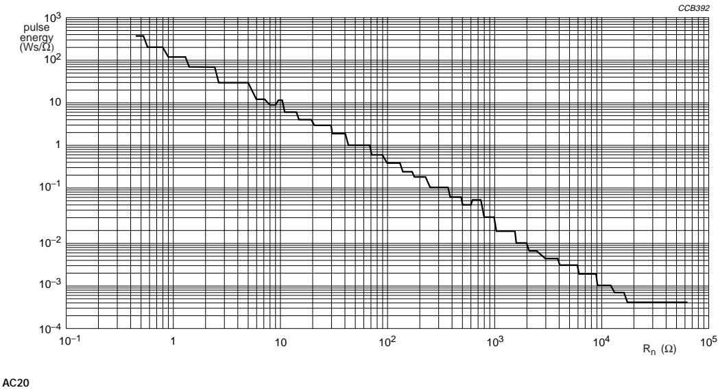
Fig.24 Pulse capability; W_s as a function of R_n .
