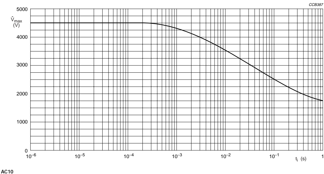
Fig.19 Pulse on a regular basis; maximum permissible peak pulse voltage ( \hat{V}_{max} ) as a function of pulse duration ( t_i ).
