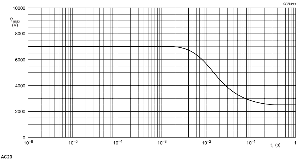
Fig.25 Pulse on a regular basis; maximum permissible peak pulse voltage ( \hat{V}_{max} ) as a function of pulse duration ( t_i ).
