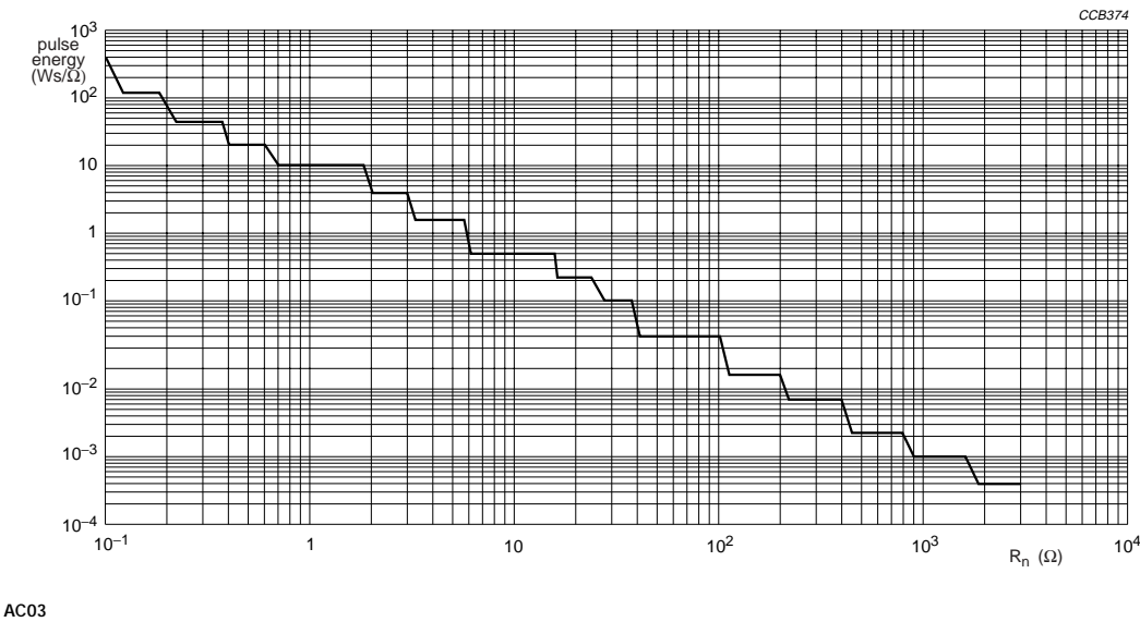
Fig.6 Pulse capability; W_s as a function of R_n .
