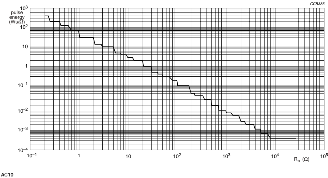
Fig.18 Pulse capability; W_s as a function of R_n .
