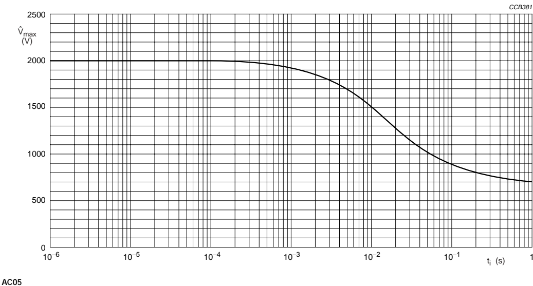
Fig.13 Pulse on a regular basis; maximum permissible peak pulse voltage ( \hat{V}_{max} ) as a function of pulse duration ( t_i ).
