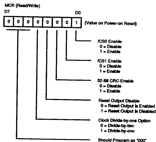
Figure 30. Misc Control Register
