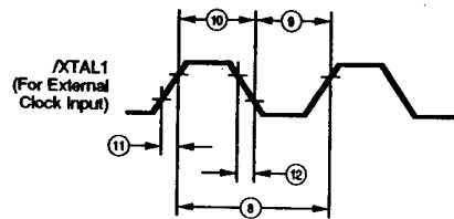
(a) XTAL1 Timing for External Clock Input
