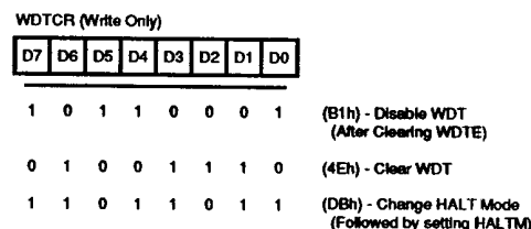
Figure 23. Watch Dog Timer Command Register
