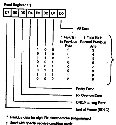
Figure 20b. SIO Read Register 1
