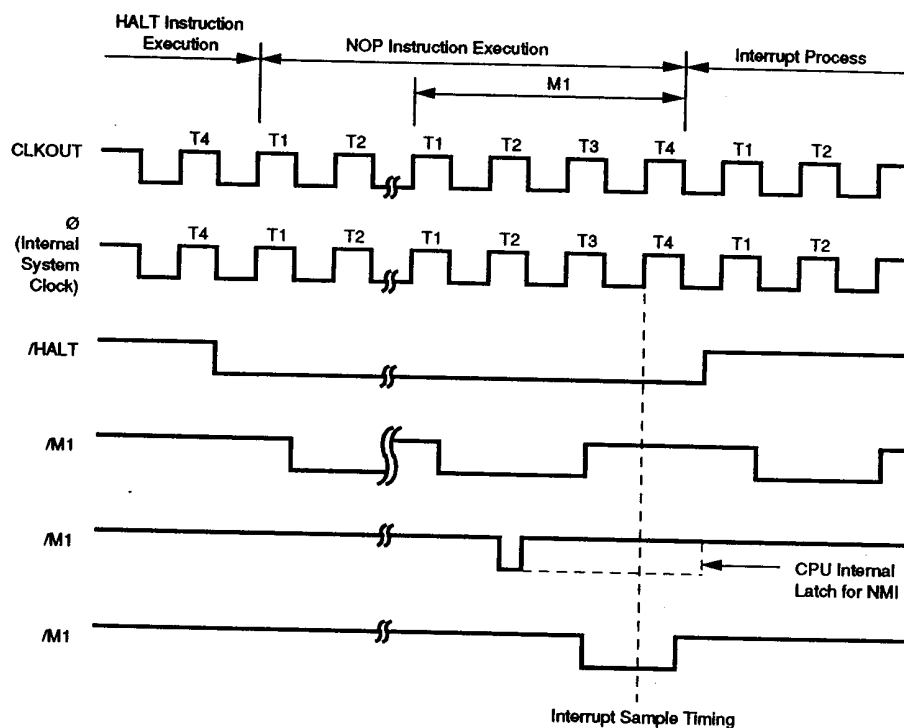
Figure 35. Halt Release Operation Timing By Interrupt Request Signal in RUN Mode
