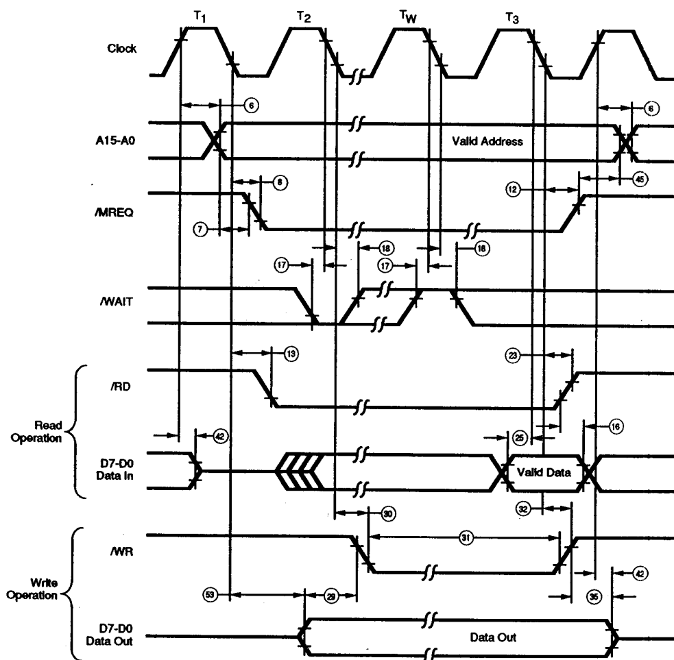
Figure 42. Memory Read or Write Cycle (See Table A)
