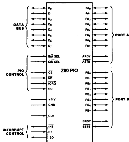
Figure 1. Pin Functions
