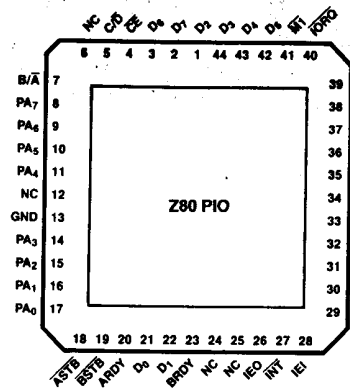
Figure 2b. 44-pin Chip Carrier, Pin Assignments
