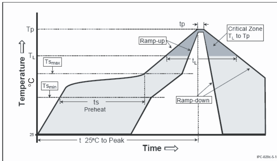
Figure 1. Classification Reflow Profile
