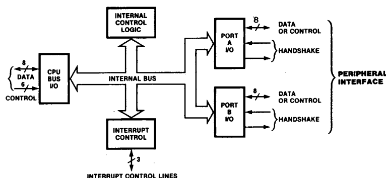
Figure 4. Block Diagram
