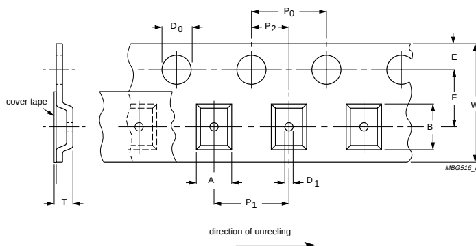
Fig. 6 Embossed tape dimension
