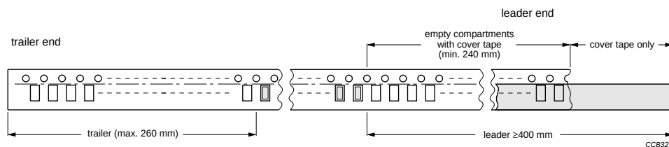
Fig. 7 Leader and trailer tape dimension
