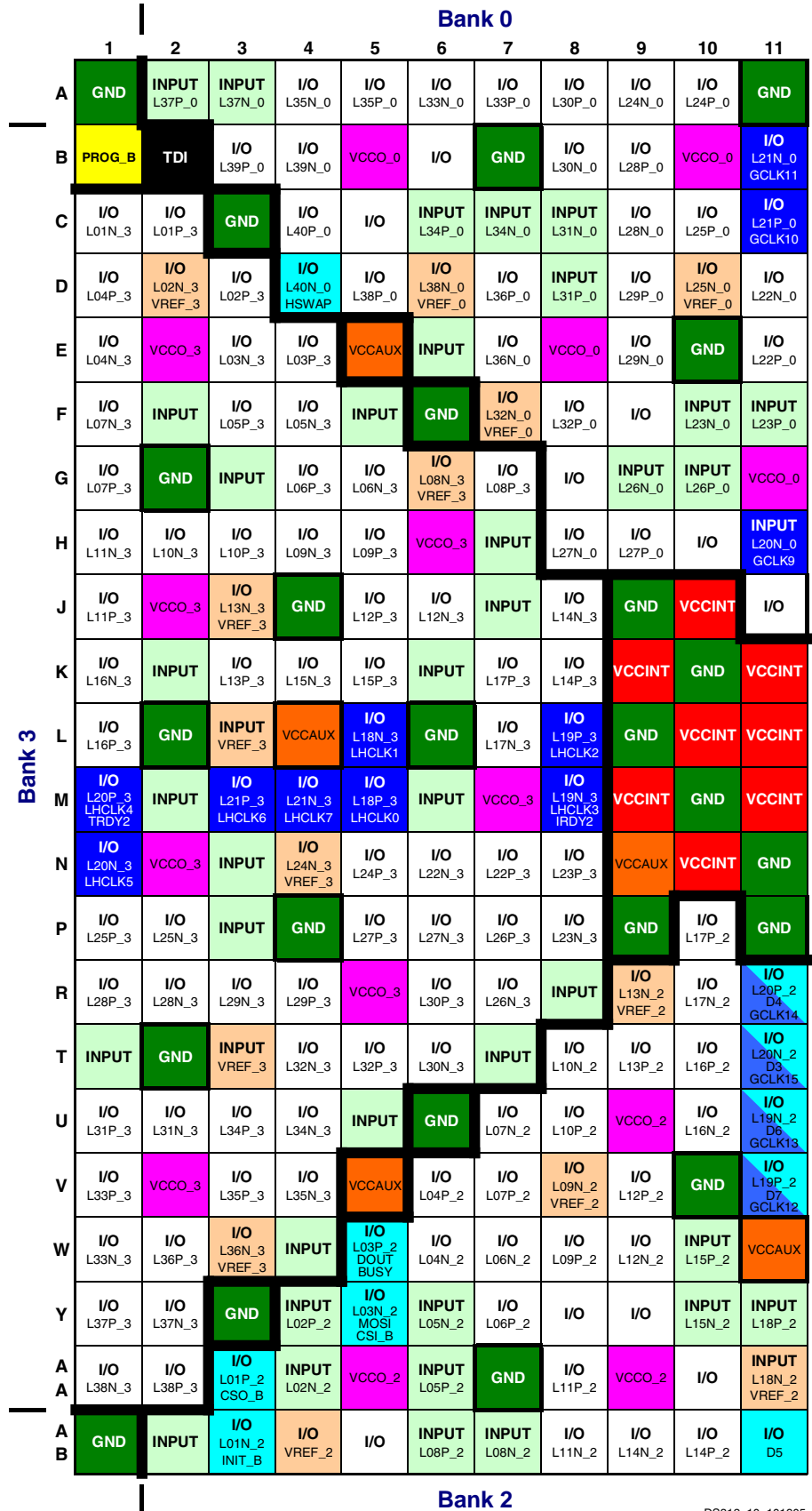
Figure 90: FG484 Package Footprint (top view)
