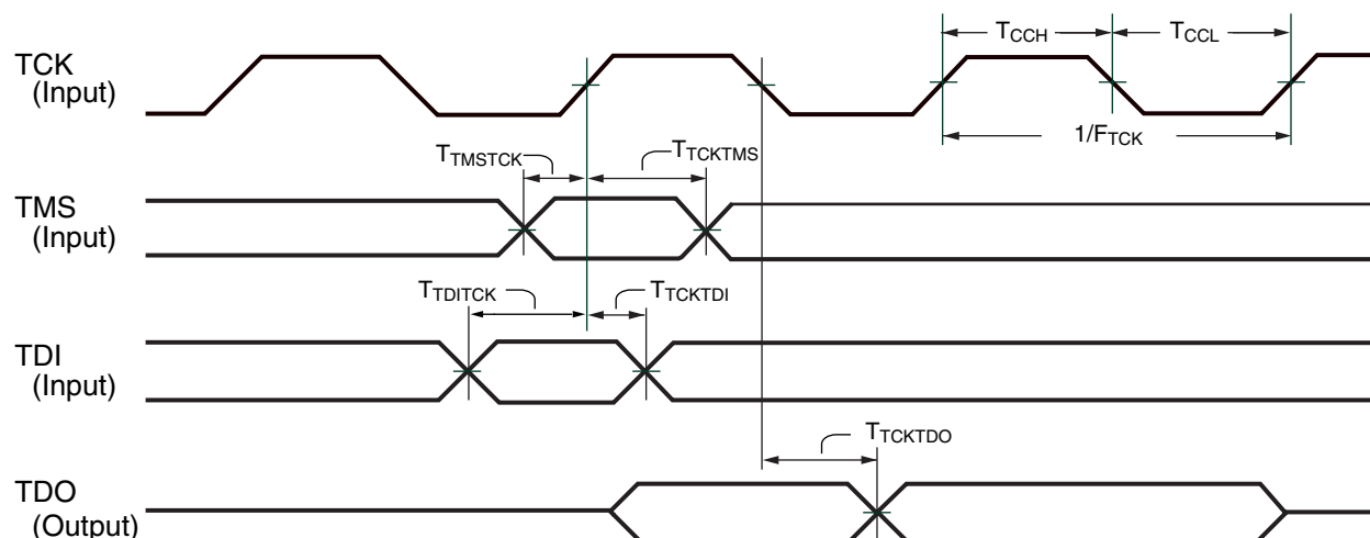
Figure 80: JTAG Waveforms
