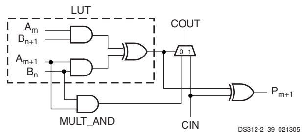
Figure 25: Using the MULT_AND for Multiplication in Carry Logic
