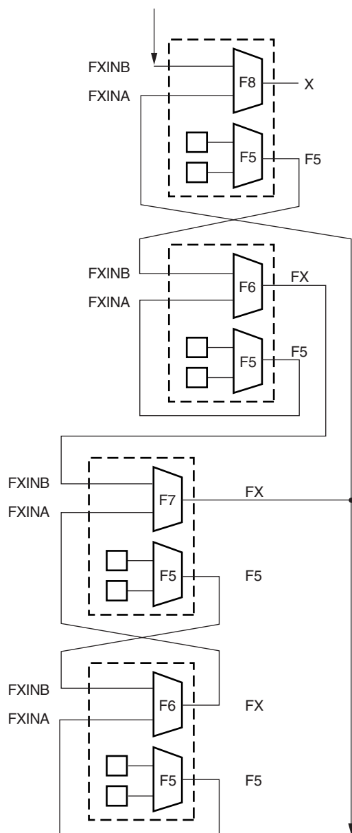
Figure 21: Muxes and Dedicated Feedback in Spartan-3E CLB
