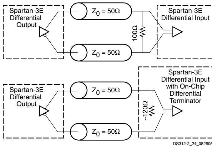
Figure 12: Differential Inputs and Outputs
