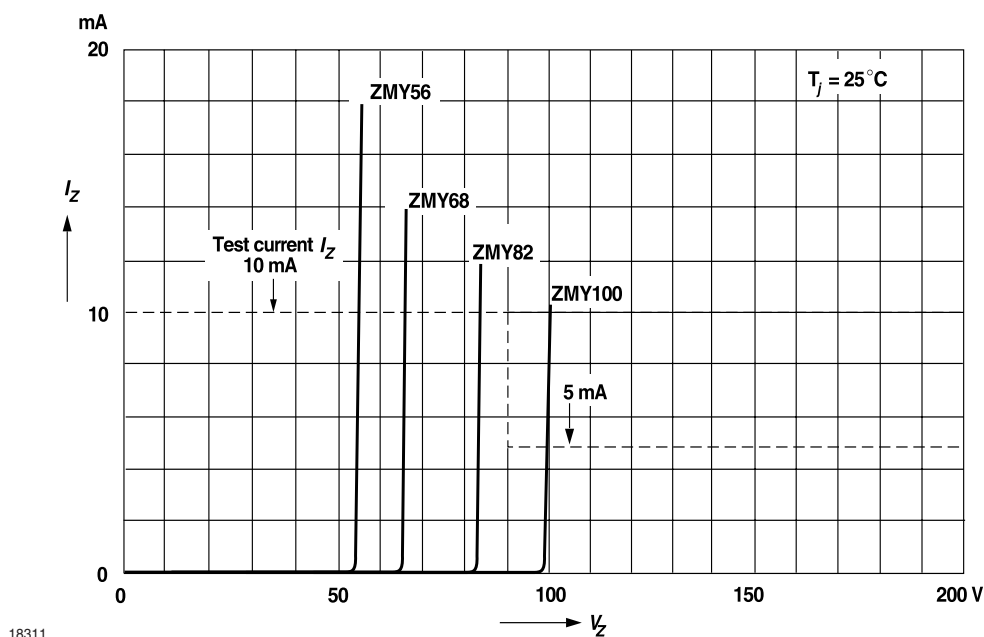
Figure 8. Breakdown Characteristics
