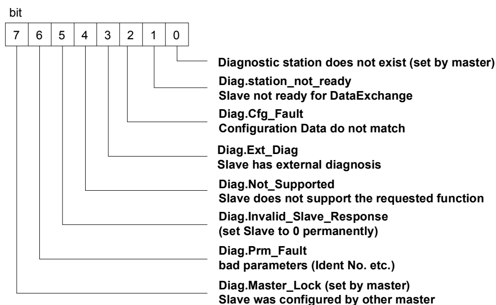
Figure 4-29 : Structure of Station_Status_1
