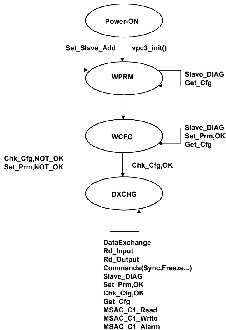
Figure 2-2 : State Machine
