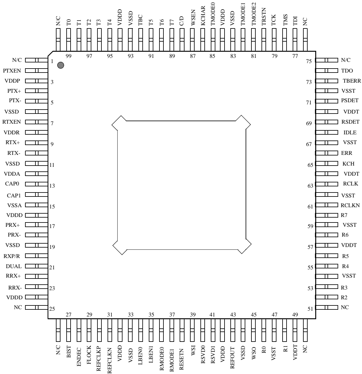
Figure 22: Pin Diagram
