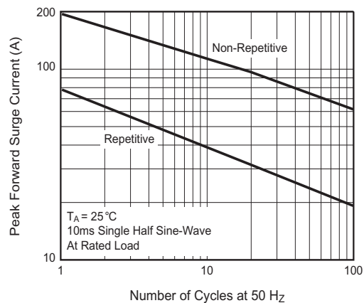
Figure 2. Maximum Peak Forward Surge Current
