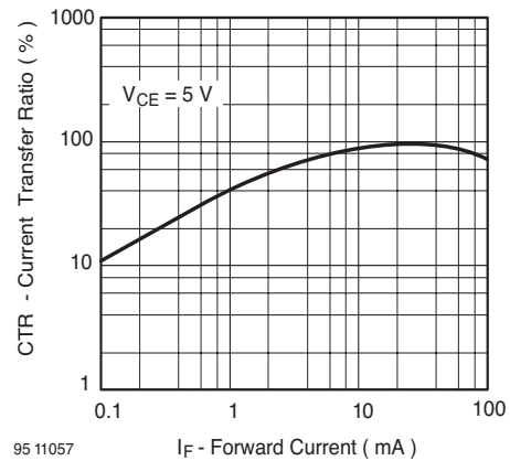
Figure 15. Current Transfer Ratio vs. Forward Current
