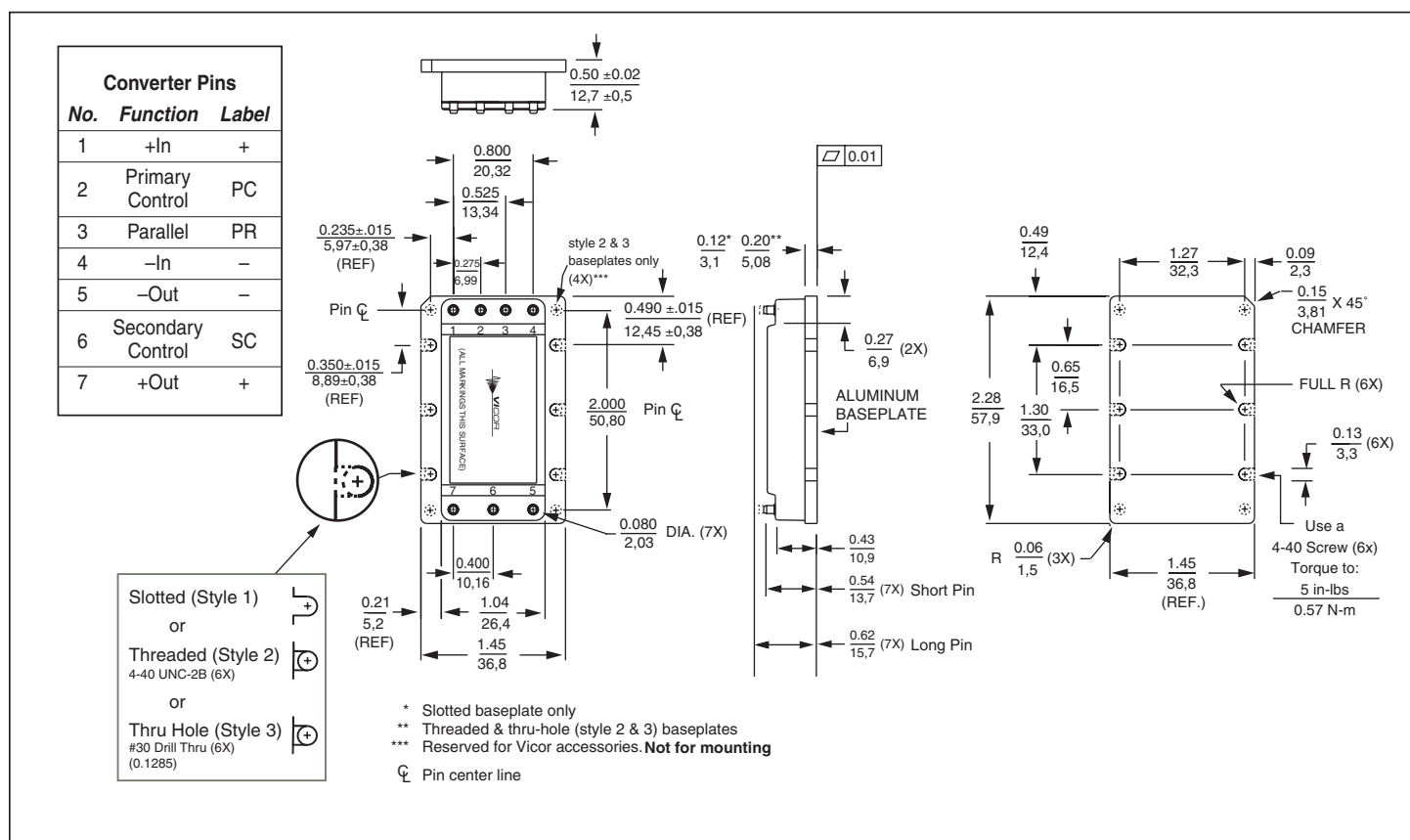
Figure 13 — Module outline
