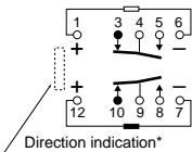
Schematic (Bottom view) 2 coil latching (Reset condition)
