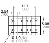
PC board pattern (Copper side view)
