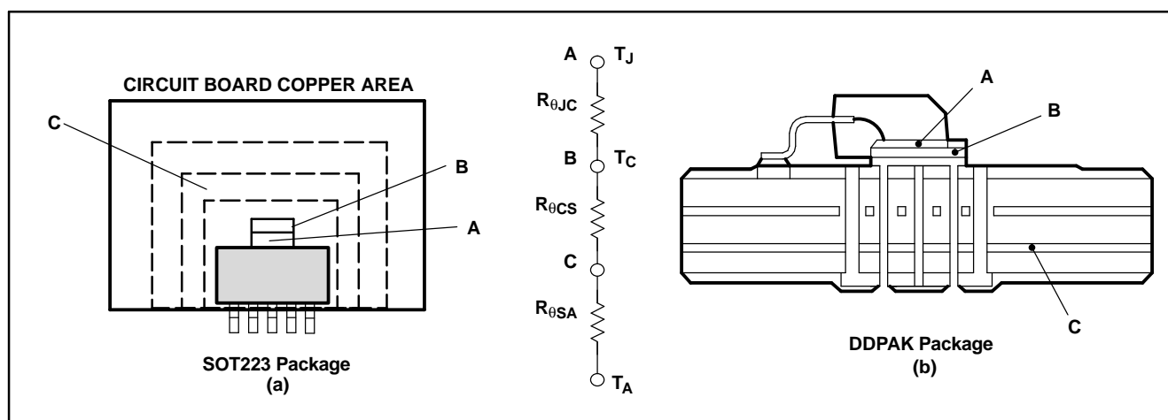
Figure 26. Thermal Resistances
