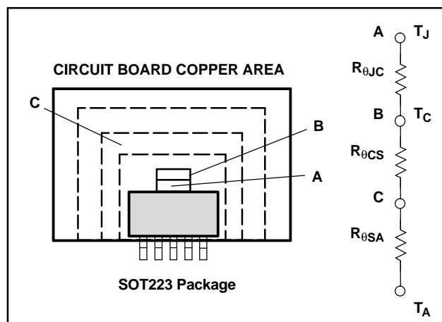
Figure 25. Thermal Resistances
